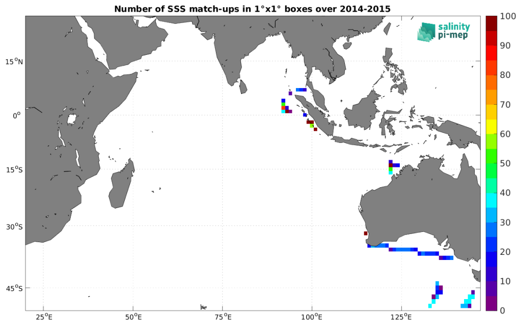
Figure 4: Number of SSS match-ups between TSG (SAMOS) SSS and the Aquarius SSS L3 OR v5 - Monthly (NASA-GSFC) SSS product for the Indian Ocean Pi-MEP region over 1^\circ \times 1^\circ boxes and for the full satellite product period.
