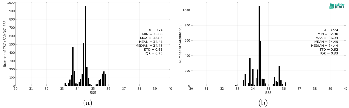
Figure 2: Histograms of SSS from TSG (SAMOS) (a) and Aquarius SSS L3 OR v5 - Monthly (NASA-GSFC) (b) considering all match-up pairs per bins of 0.1 over the Indian Ocean Pi-MEP region and for the full satellite product period.
