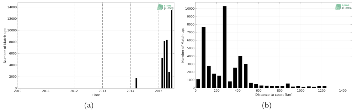
Figure 1: Number of match-ups between TSG (SAMOS) and Aquarius SSS L3 OR v5 - Monthly (NASA-GSFC) SSS as a function of time (a) and as function of the distance to coast (b) over the Indian Ocean Pi-MEP region and for the full satellite product period.
