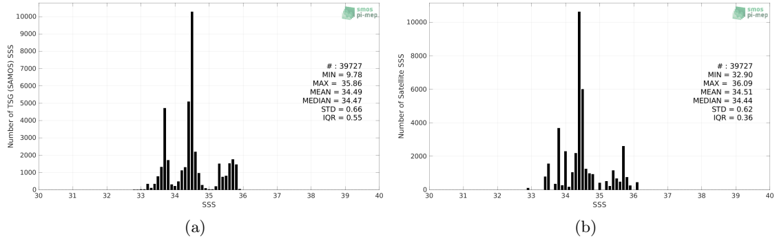
Figure 2: Histograms of SSS from TSG (SAMOS) (a) and Aquarius SSS L3 OR v5 - Monthly (NASA-GSFC) (b) considering all match-up pairs per bins of 0.1 over the Indian Ocean Pi-MEP region and for the full satellite product period.
