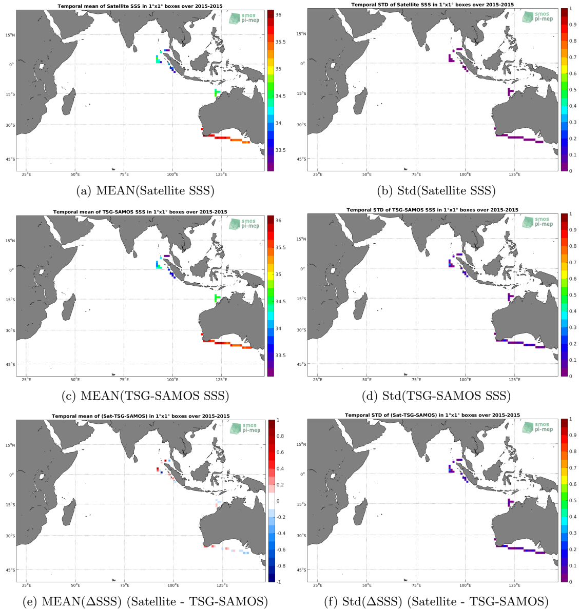
Figure 6: Temporal mean (left) and Std (right) of SSS from Aquarius-L3-OR-V5-MONTHLY-1DEG (top), TSG-SAMOS (middle), and of \Delta SSS (Satellite - TSG-SAMOS). Only match-up pairs are used to generate these maps.
