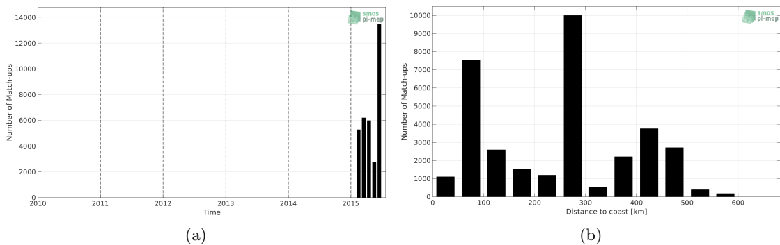
Figure 1: Number of match-ups between TSG-SAMOS and Aquarius-L3-OR-V5-MONTHLY-1DEG SSS as a function of time (a) and as function of the distance to coast (b) over the Indian Ocean Pi-MEP region and for the full satellite product period.
