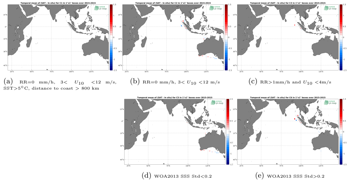
Figure 12: Temporal mean gridded over spatial boxes of size 1^\circ \times 1^\circ of \Delta SSS (Aquarius-L3-OR-V5-MONTHLY-1DEG - TSG-SAMOS) for 5 different subdatasets corresponding to:RR=0 mm/h, 3 < U_{10} < 12 m/s, SST >5^\circ C, distance to coast > 800 km (a), RR=0 mm/h, 3 < U_{10} < 12 m/s (b), RR >1 mm/h and U_{10} < 4 m/s (c), WOA2013 SSS Std <0.2 (d), WOA2013 SSS Std >0.2 (e).
