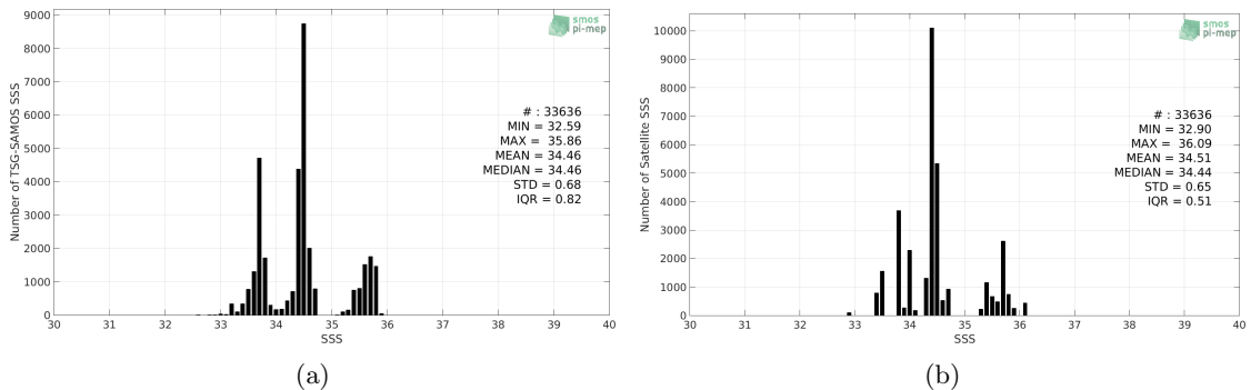
Figure 2: Histograms of SSS from TSG-SAMOS (a) and Aquarius-L3-OR-V5-MONTHLY-1DEG (b) considering all match-up pairs per bins of 0.1 over the Indian Ocean Pi-MEP region and for the full satellite product period.
