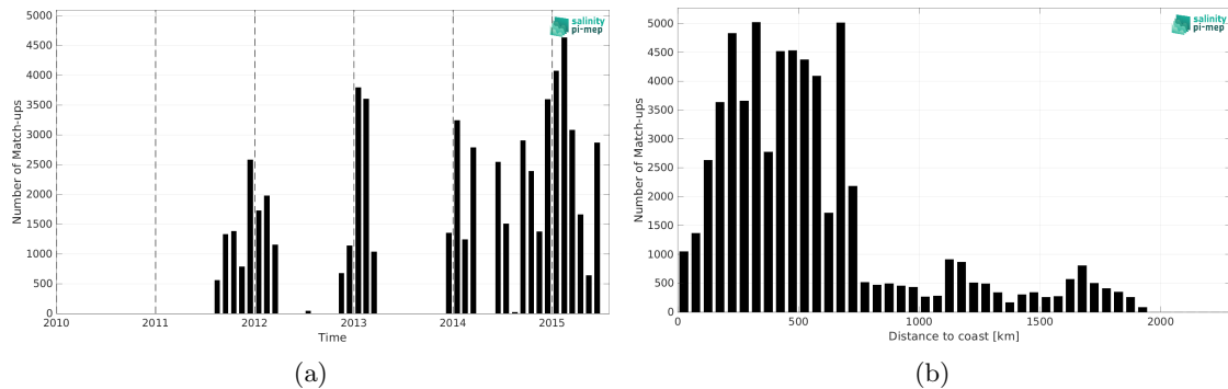
Figure 2: Number of match-ups between TSG (LEGOS-DM) and Aquarius SSS L3 OR v5 - Monthly (NASA-GSFC) SSS as a function of time (a) and as function of the distance to coast (b) over the Indian Ocean Pi-MEP region and for the full satellite product period.
