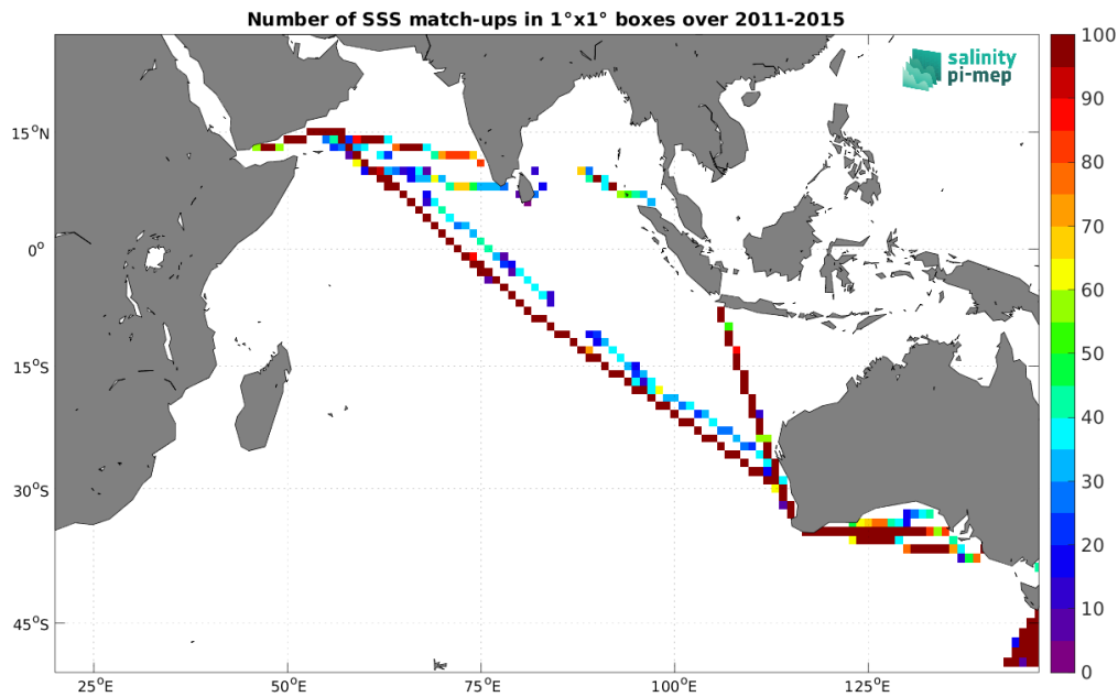
Figure 5: Number of SSS match-ups between TSG (LEGOS-DM) SSS and the Aquarius SSS L3 OR v5 - Monthly (NASA-GSFC) SSS product for the Indian Ocean Pi-MEP region over 1^\circ \times 1^\circ boxes and for the full satellite product period.
