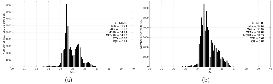
Figure 3: Histograms of SSS from TSG (LEGOS-DM) (a) and Aquarius SSS L3 OR v5 - Monthly (NASA-GSFC) (b) considering all match-up pairs per bins of 0.1 over the Indian Ocean Pi-MEP region and for the full satellite product period.
