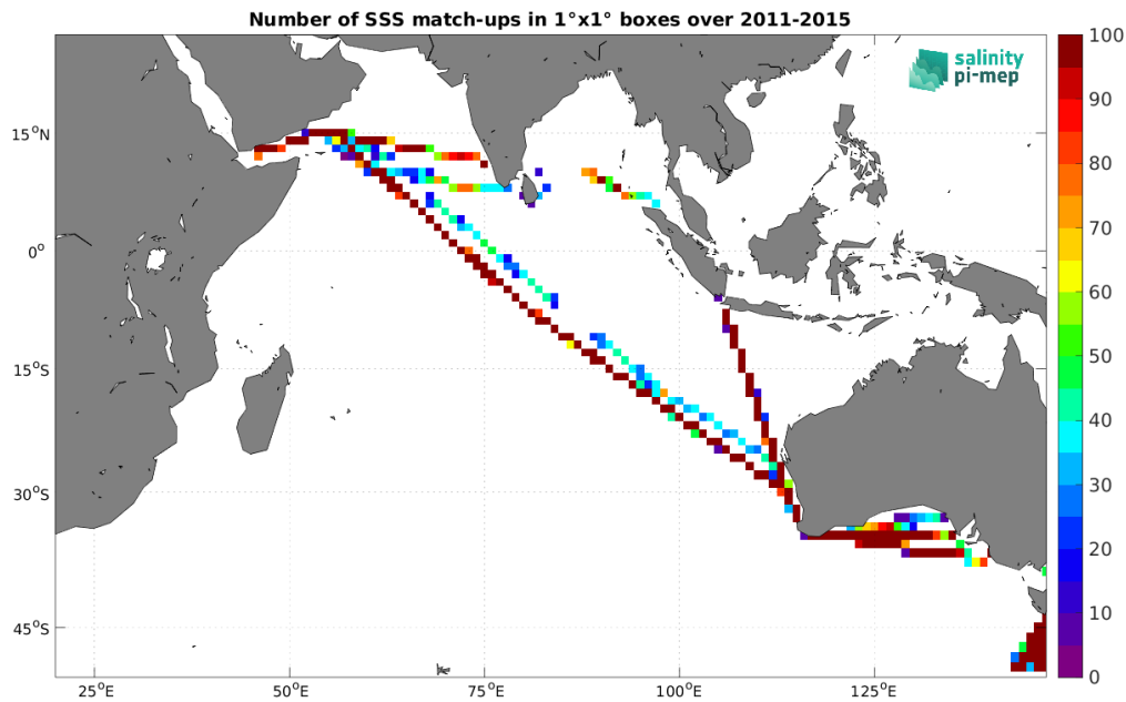
Figure 4: Number of SSS match-ups between TSG (LEGOS-DM) SSS and the Aquarius SSS L3 OR v5 - Monthly (NASA-GSFC) SSS product for the Indian Ocean Pi-MEP region over 1^\circ \times 1^\circ boxes and for the full satellite product period.
