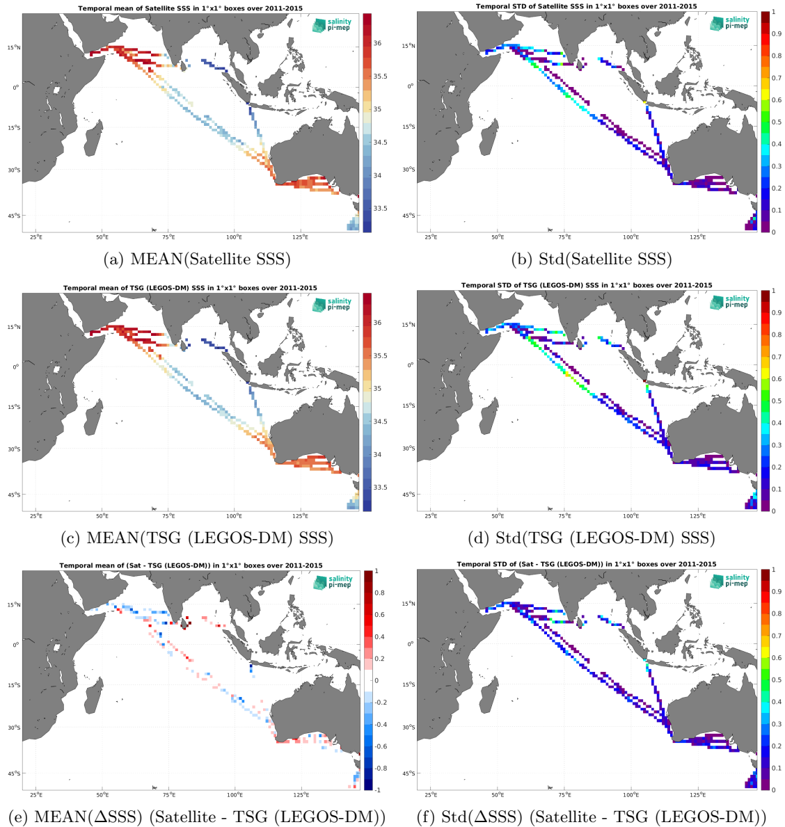
Figure 6: Temporal mean (left) and Std (right) of SSS from Aquarius SSS L3 OR v5 - Monthly (NASA-GSFC) (top), TSG (LEGOS-DM) ( in situ ) dataset (middle), and of \Delta SSS (Satellite - TSG (LEGOS-DM)). Only match-up pairs are used to generate these maps.
