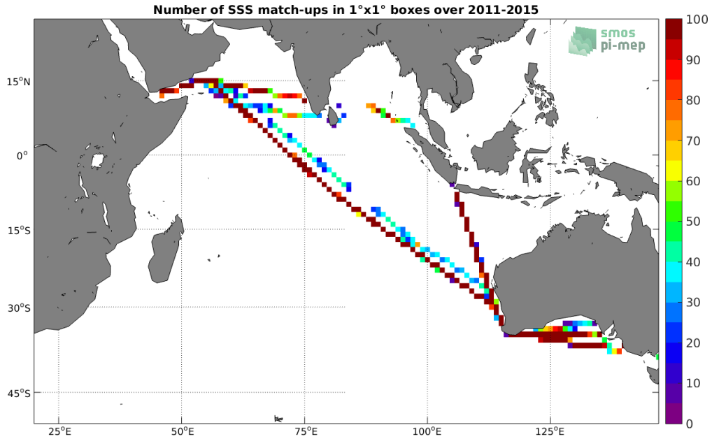
Figure 4: Number of SSS match-ups between TSG (LEGOS-DM) SSS and the Aquarius SSS L3 OR v5 - Monthly (NASA-GSFC) SSS product for the Indian Ocean Pi-MEP region over 1^\circ \times 1^\circ boxes and for the full satellite product period.
