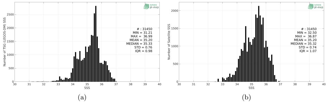
Figure 2: Histograms of SSS from TSG (LEGOS-DM) (a) and Aquarius SSS L3 OR v5 - Monthly (NASA-GSFC) (b) considering all match-up pairs per bins of 0.1 over the Indian Ocean Pi-MEP region and for the full satellite product period.
