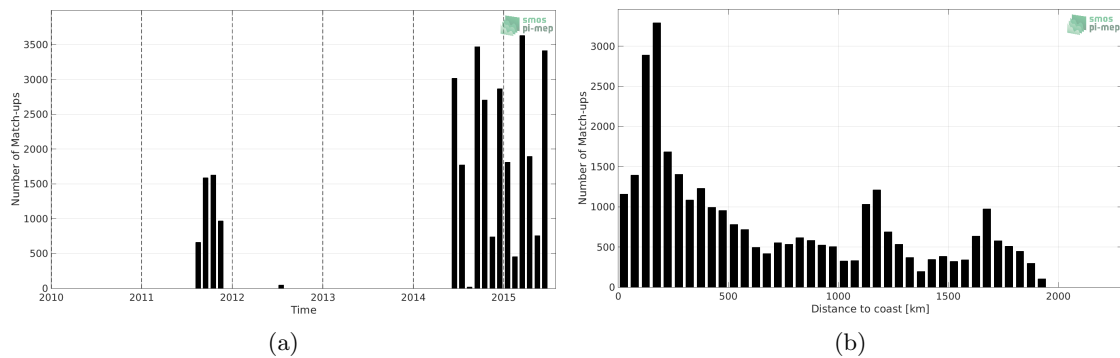
Figure 1: Number of match-ups between TSG (LEGOS-DM) and Aquarius SSS L3 OR v5 - Monthly (NASA-GSFC) SSS as a function of time (a) and as function of the distance to coast (b) over the Indian Ocean Pi-MEP region and for the full satellite product period.
