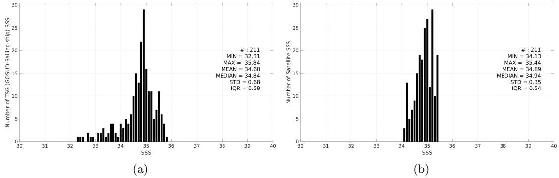
Figure 3: Histograms of SSS from TSG (GOSUD-Sailing-ship) (a) and Aquarius SSS L3 OR v5 - Monthly (NASA-GSFC) (b) considering all match-up pairs per bins of 0.1 over the Indian Ocean Pi-MEP region and for the full satellite product period.
