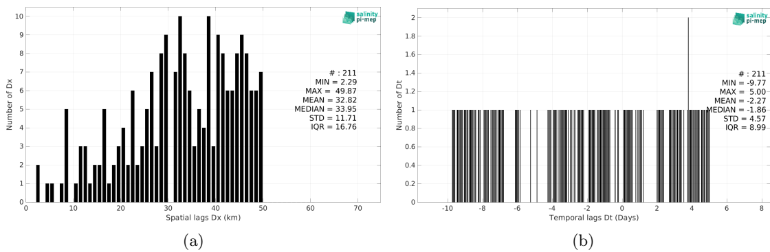
Figure 6: Histograms of the spatial (a) and temporal (b) lags between the location/time of the TSG (GOSUD-Sailing-ship) measurement and the date of the corresponding Aquarius SSS L3 OR v5 - Monthly (NASA-GSFC) SSS pixel.
