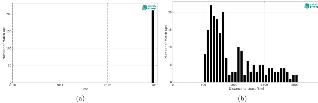
Figure 2: Number of match-ups between TSG (GOSUD-Sailing-ship) and Aquarius SSS L3 OR v5 - Monthly (NASA-GSFC) SSS as a function of time (a) and as function of the distance to coast (b) over the Indian Ocean Pi-MEP region and for the full satellite product period.
