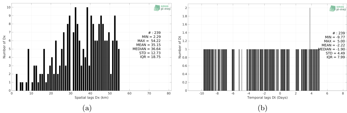
Figure 5: Histograms of the spatial (a) and temporal (b) lags between the location/time of the TSG (GOSUD-Sailing-ship) measurement and the date of the corresponding Aquarius SSS L3 OR v5 - Monthly (NASA-GSFC) SSS pixel.
