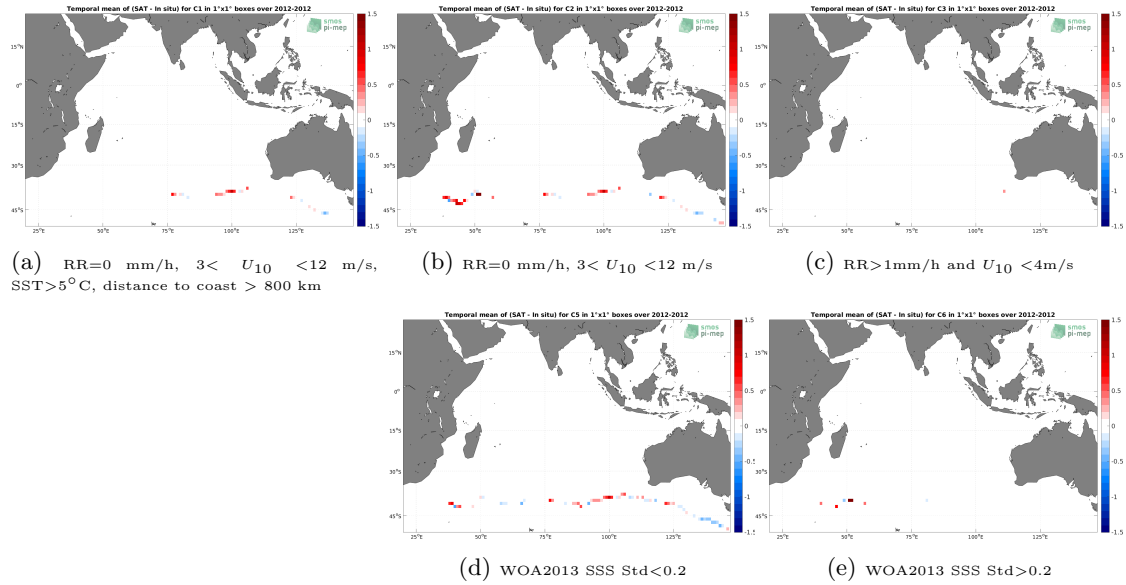
Figure 12: Temporal mean gridded over spatial boxes of size 1^{\circ}\times 1^{\circ} of \Delta SSS (Aquarius SSS L3 OR v5 - Monthly (NASA-GSFC) - TSG (GOSUD-Sailing-ship)) for 5 different subdatasets corresponding to:RR=0 mm/h, 3 < U_{10} < 12 m/s, SST >5^{\circ}\text{C} , distance to coast > 800 km (a), RR=0 mm/h, 3 < U_{10} < 12 m/s (b), RR >1 mm/h and U_{10} < 4 m/s (c), WOA2013 SSS Std <0.2 (d), WOA2013 SSS Std >0.2 (e).
