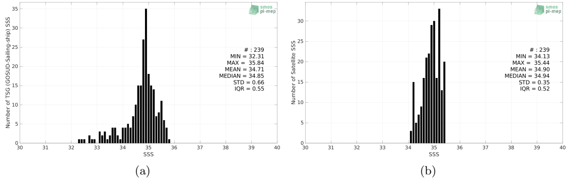
Figure 2: Histograms of SSS from TSG (GOSUD-Sailing-ship) (a) and Aquarius SSS L3 OR v5 - Monthly (NASA-GSFC) (b) considering all match-up pairs per bins of 0.1 over the Indian Ocean Pi-MEP region and for the full satellite product period.
