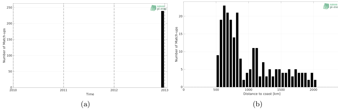
Figure 1: Number of match-ups between TSG (GOSUD-Sailing-ship) and Aquarius SSS L3 OR v5 - Monthly (NASA-GSFC) SSS as a function of time (a) and as function of the distance to coast (b) over the Indian Ocean Pi-MEP region and for the full satellite product period.
