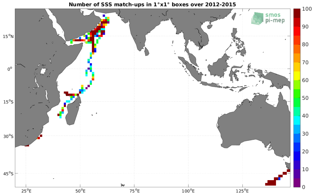
Figure 4: Number of SSS match-ups between TSG (GOSUD-Research-vessel) SSS and the Aquarius SSS L3 OR v5 - Monthly (NASA-GSFC) SSS product for the Indian Ocean Pi-MEP region over 1^\circ \times 1^\circ boxes and for the full satellite product period.
