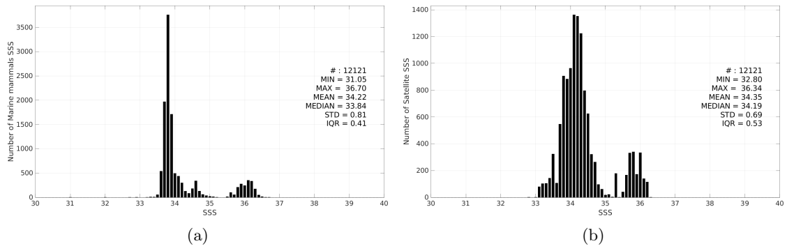
Figure 3: Histograms of SSS from Marine mammals (a) and Aquarius SSS L3 OR v5 - Monthly (NASA-GSFC) (b) considering all match-up pairs per bins of 0.1 over the Indian Ocean Pi-MEP region and for the full satellite product period.
