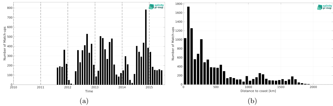
Figure 2: Number of match-ups between Marine mammals and Aquarius SSS L3 OR v5 - Monthly (NASA-GSFC) SSS as a function of time (a) and as function of the distance to coast (b) over the Indian Ocean Pi-MEP region and for the full satellite product period.
