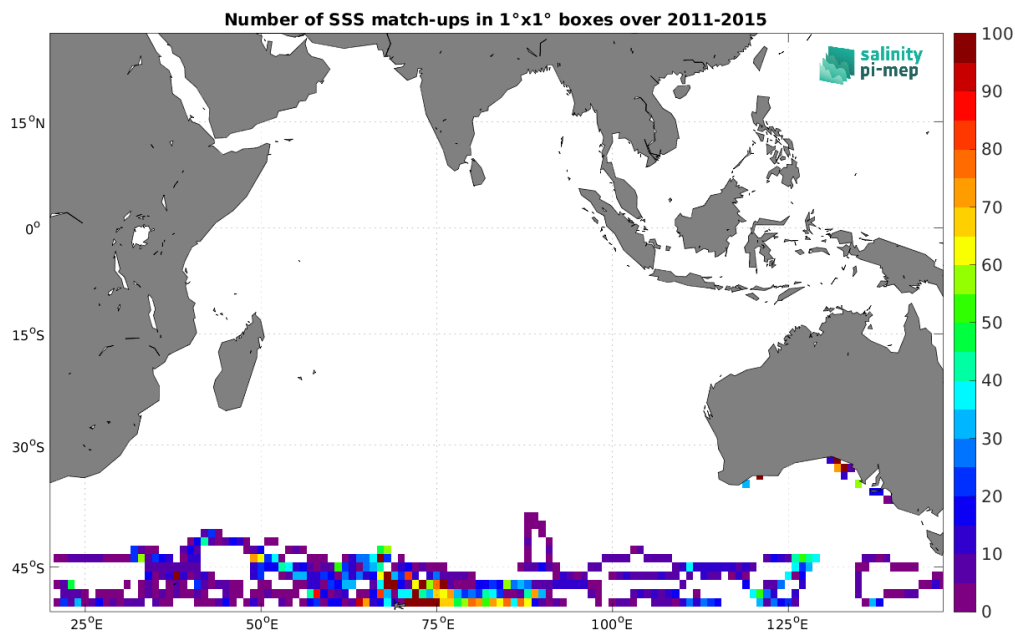
Figure 5: Number of SSS match-ups between Marine mammals SSS and the Aquarius SSS L3 OR v5 - Monthly (NASA-GSFC) SSS product for the Indian Ocean Pi-MEP region over 1^\circ \times 1^\circ boxes and for the full satellite product period.
