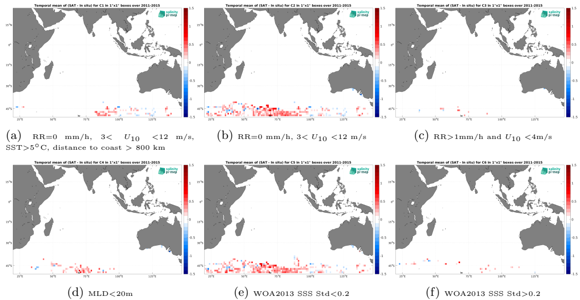
Figure 14: Temporal mean gridded over spatial boxes of size 1^\circ \times 1^\circ of \Delta SSS (Aquarius SSS L3 OR v5 - Monthly (NASA-GSFC) - Marine mammals) for 6 different subdatasets corresponding to: RR=0 mm/h, 3 < U_{10} < 12 m/s, SST > 5°C, distance to coast > 800 km (a), RR=0 mm/h, 3 < U_{10} < 12 m/s (b), RR > 1mm/h and U_{10} < 4 m/s (c), MLD < 20m (d), WOA2013 SSS Std < 0.2 (e), WOA2013 SSS Std > 0.2 (f).
