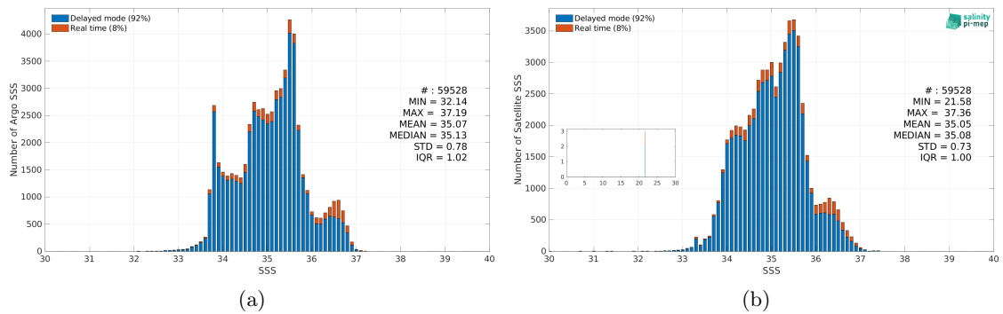
Figure 3: Histograms of SSS from Argo (a) and Aquarius SSS L3 OR v5 - Monthly (NASA-GSFC) (b) considering all match-up pairs per bins of 0.1 over the Indian Ocean Pi-MEP region and for the full satellite product period.
