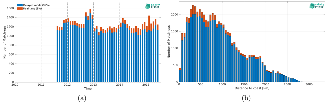
Figure 2: Number of match-ups between Argo and Aquarius SSS L3 OR v5 - Monthly (NASA-GSFC) SSS as a function of time (a) and as function of the distance to coast (b) over the Indian Ocean Pi-MEP region and for the full satellite product period.
