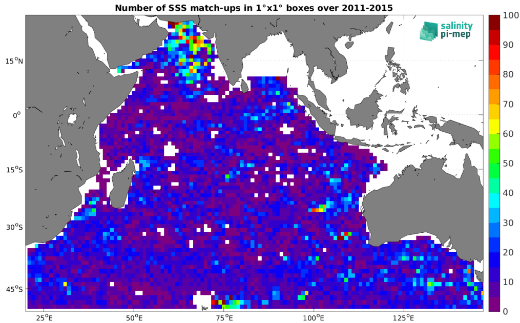
Figure 5: Number of SSS match-ups between Argo SSS and the Aquarius SSS L3 OR v5 - Monthly (NASA-GSFC) SSS product for the Indian Ocean Pi-MEP region over 1^\circ \times 1^\circ boxes and for the full satellite product period.
