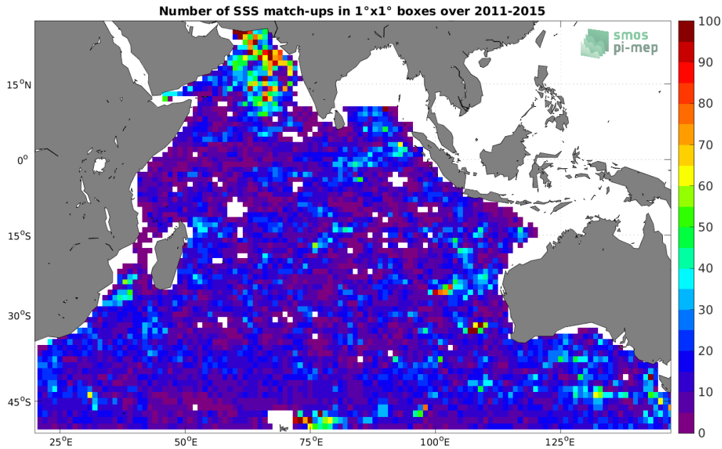
Figure 4: Number of SSS match-ups between Argo SSS and the Aquarius SSS L3 OR v5 - Monthly (NASA-GSFC) SSS product for the Indian Ocean Pi-MEP region over 1^\circ \times 1^\circ boxes and for the full satellite product period.
