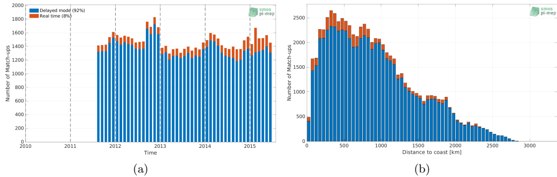
Figure 1: Number of match-ups between Argo and Aquarius SSS L3 OR v5 - Monthly (NASA-GSFC) SSS as a function of time (a) and as function of the distance to coast (b) over the Indian Ocean Pi-MEP region and for the full satellite product period.
