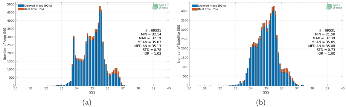
Figure 2: Histograms of SSS from Argo (a) and Aquarius SSS L3 OR v5 - Monthly (NASA-GSFC) (b) considering all match-up pairs per bins of 0.1 over the Indian Ocean Pi-MEP region and for the full satellite product period.
