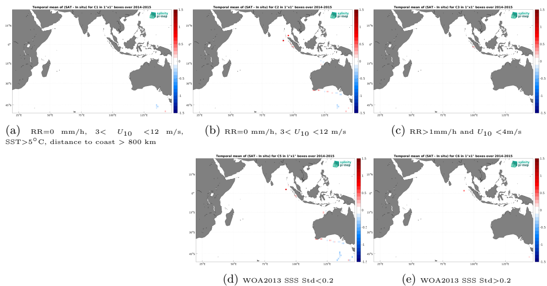
Figure 14: Temporal mean gridded over spatial boxes of size 1^\circ \times 1^\circ of \Delta\text{SSS} (Aquarius SSS L3 OR v5 - Monthly - Rain mask (NASA-GSFC) - TSG (SAMOS)) for 5 different subdatasets corresponding to:RR=0 mm/h, 3 < U_{10} < 12 m/s, SST >5^\circ\text{C} , distance to coast > 800 km (a), RR=0 mm/h, 3 < U_{10} < 12 m/s (b), RR >1 mm/h and U_{10} < 4 m/s (c), WOA2013 SSS Std <0.2 (d), WOA2013 SSS Std >0.2 (e).
