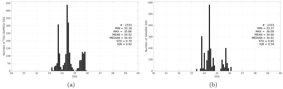
Figure 3: Histograms of SSS from TSG (SAMOS) (a) and Aquarius SSS L3 OR v5 - Monthly - Rain mask (NASA-GSFC) (b) considering all match-up pairs per bins of 0.1 over the Indian Ocean Pi-MEP region and for the full satellite product period.
