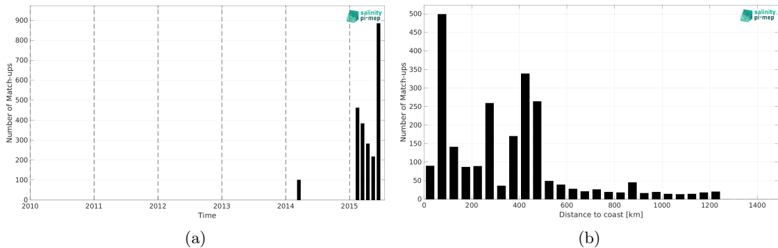
Figure 2: Number of match-ups between TSG (SAMOS) and Aquarius SSS L3 OR v5 - Monthly - Rain mask (NASA-GSFC) SSS as a function of time (a) and as function of the distance to coast (b) over the Indian Ocean Pi-MEP region and for the full satellite product period.
