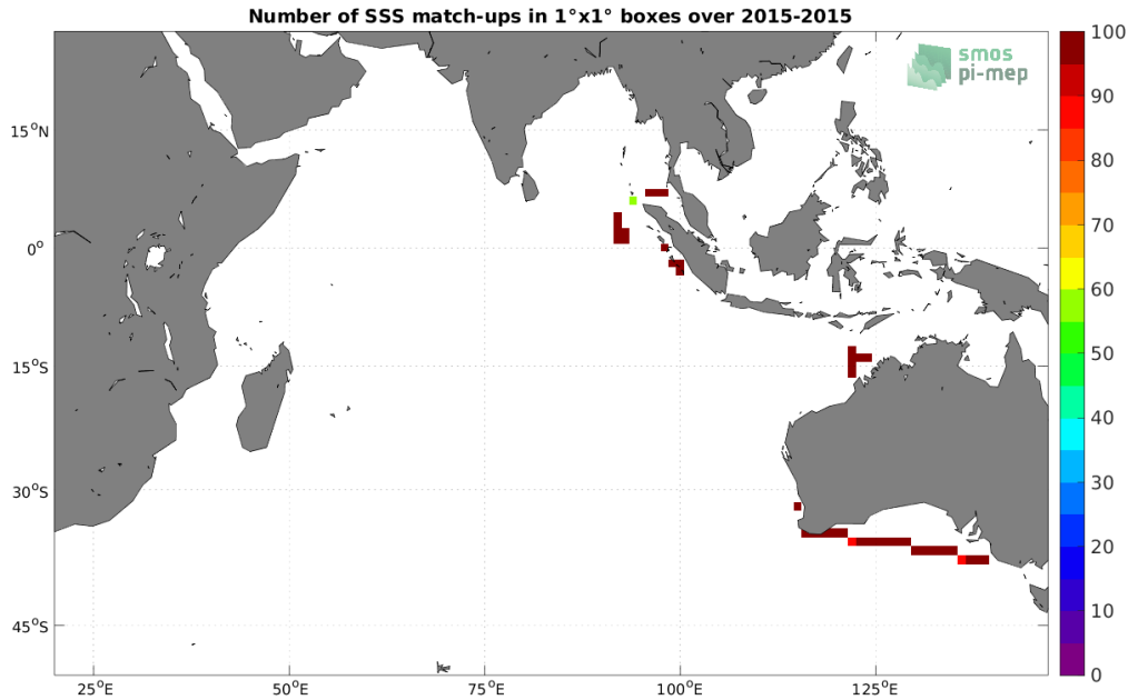
Figure 4: Number of SSS match-ups between TSG (SAMOS) SSS and the Aquarius SSS L3 OR v5 - Monthly - Rain mask (NASA-GSFC) SSS product for the Indian Ocean Pi-MEP region over 1°x1° boxes and for the full satellite product period.
