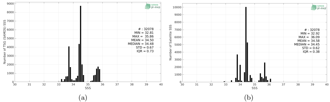
Figure 2: Histograms of SSS from TSG (SAMOS) (a) and Aquarius SSS L3 OR v5 - Monthly - Rain mask (NASA-GSFC) (b) considering all match-up pairs per bins of 0.1 over the Indian Ocean Pi-MEP region and for the full satellite product period.
