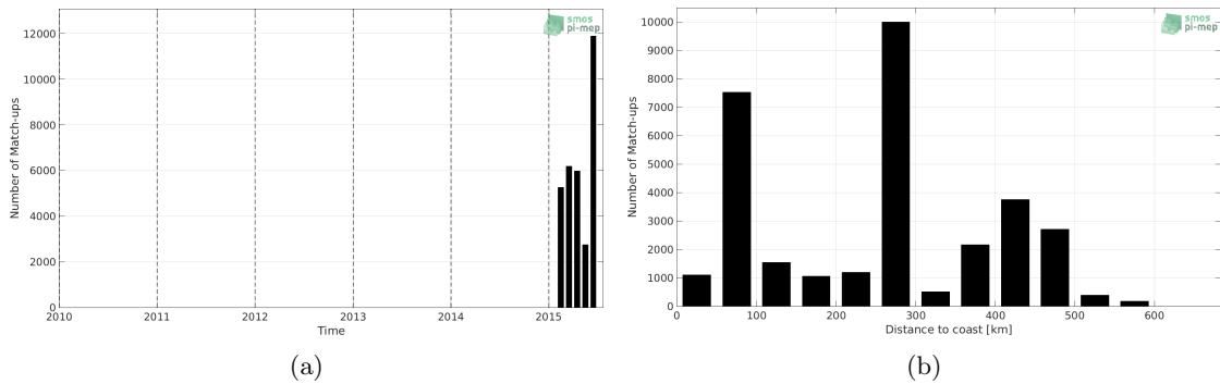
Figure 1: Number of match-ups between TSG-SAMOS and Aquarius-L3-OR-V5-MONTHLY-RAIN-MASK-1DEG SSS as a function of time (a) and as function of the distance to coast (b) over the Indian Ocean Pi-MEP region and for the full satellite product period.
