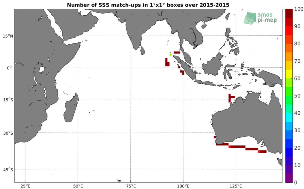
Figure 4: Number of SSS match-ups between TSG-SAMOS SSS and the Aquarius-L3-OR-V5-MONTHLY-RAIN-MASK-1DEG SSS product for the Indian Ocean Pi-MEP region over 1^\circ \times 1^\circ boxes and for the full satellite product period.
