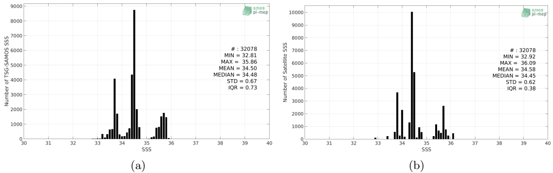
Figure 2: Histograms of SSS from TSG-SAMOS (a) and Aquarius-L3-OR-V5-MONTHLY-RAIN-MASK-1DEG (b) considering all match-up pairs per bins of 0.1 over the Indian Ocean Pi-MEP region and for the full satellite product period.
