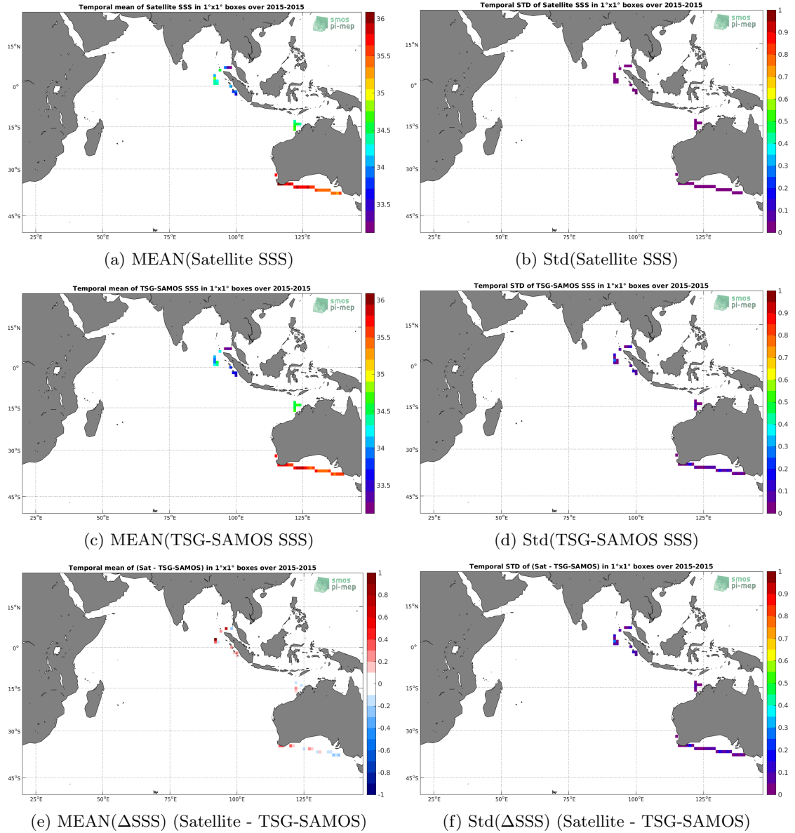
Figure 6: Temporal mean (left) and Std (right) of SSS from Aquarius-L3-OR-V5-MONTHLY-RAIN-MASK-1DEG (top), TSG-SAMOS (middle), and of \Delta SSS (Satellite - TSG-SAMOS). Only match-up pairs are used to generate these maps.
