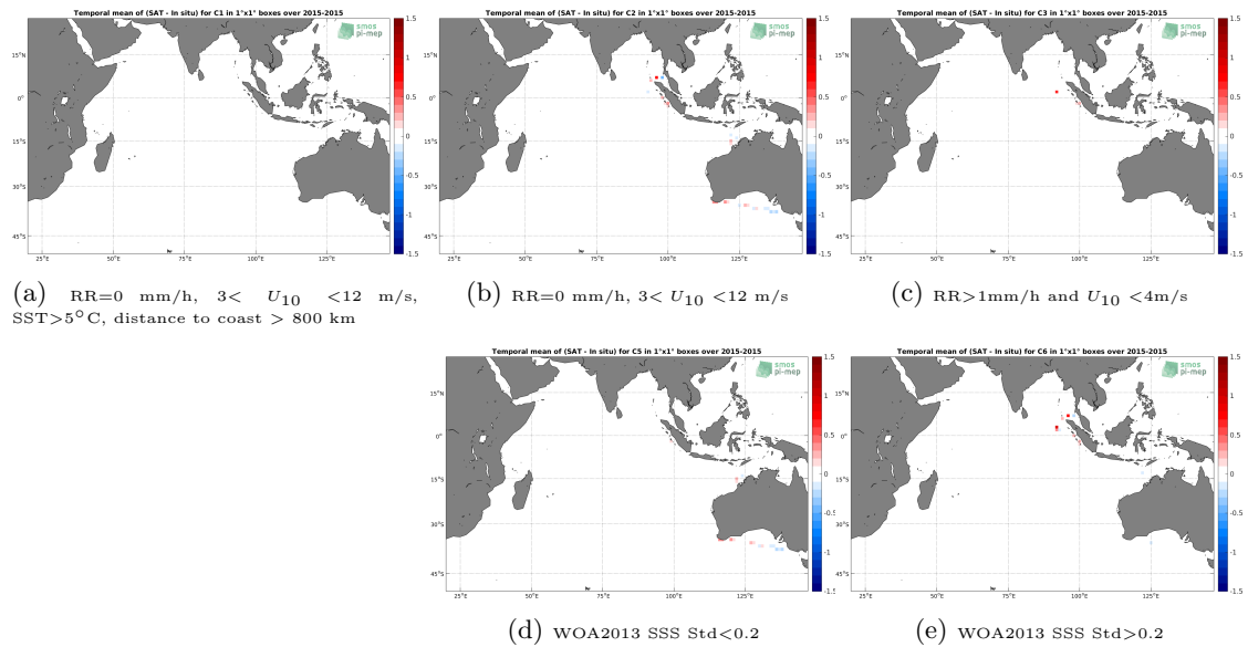
Figure 12: Temporal mean gridded over spatial boxes of size 1^\circ \times 1^\circ of \Delta SSS (Aquarius-L3-OR-V5-MONTHLY-RAIN-MASK-1DEG - TSG-SAMOS) for 5 different subdatasets corresponding to:RR=0 mm/h, 3 < U_{10} < 12 m/s, SST >5^\circ C, distance to coast > 800 km (a), RR=0 mm/h, 3 < U_{10} < 12 m/s (b), RR >1 mm/h and U_{10} < 4 m/s (c), WOA2013 SSS Std <0.2 (d), WOA2013 SSS Std >0.2 (e).
