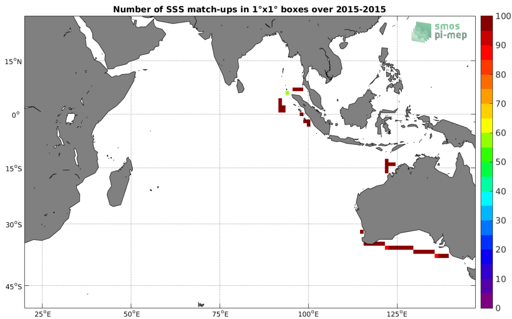
Figure 4: Number of SSS match-ups between TSG-SAMOS SSS and the Aquarius-L3-OR-V5-MONTHLY-RAIN-MASK-1DEG SSS product for the Indian Ocean Pi-MEP region over 1^\circ \times 1^\circ boxes and for the full satellite product period.
