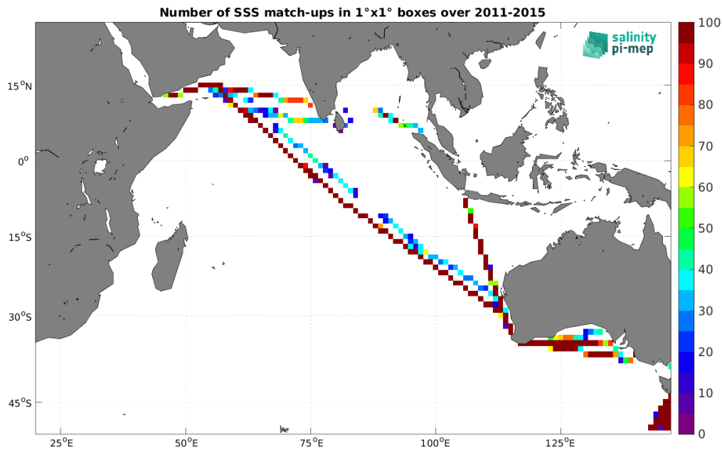
Figure 5: Number of SSS match-ups between TSG (LEGOS-DM) SSS and the Aquarius SSS L3 OR v5 - Monthly - Rain mask (NASA-GSFC) SSS product for the Indian Ocean Pi-MEP region over 1^\circ \times 1^\circ boxes and for the full satellite product period.
