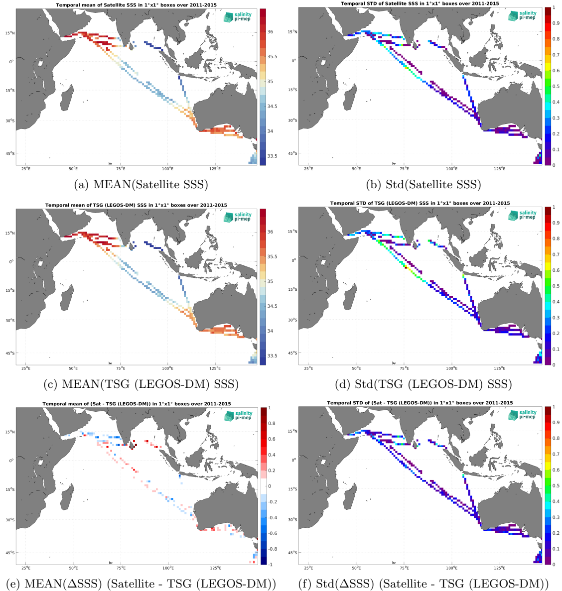
Figure 7: Temporal mean (left) and Std (right) of SSS from Aquarius SSS L3 OR v5 - Monthly - Rain mask (NASA-GSFC) (top), TSG (LEGOS-DM) (middle), and of \Delta SSS (Satellite - TSG (LEGOS-DM)). Only match-up pairs are used to generate these maps.
