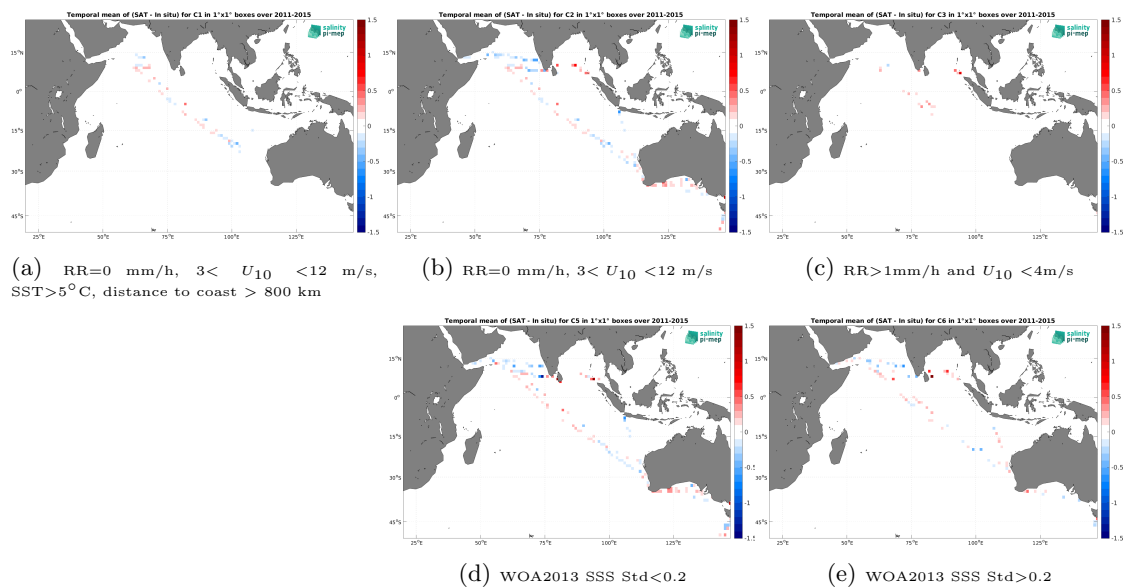
Figure 14: Temporal mean gridded over spatial boxes of size 1^\circ \times 1^\circ of \Delta SSS (Aquarius SSS L3 OR v5 - Monthly - Rain mask (NASA-GSFC) - TSG (LEGOS-DM)) for 5 different subdatasets corresponding to:RR=0 mm/h, 3 < U_{10} < 12 m/s, SST >5^\circ C, distance to coast > 800 km (a), RR=0 mm/h, 3 < U_{10} < 12 m/s (b), RR >1 mm/h and U_{10} < 4 m/s (c), WOA2013 SSS Std <0.2 (d), WOA2013 SSS Std >0.2 (e).
