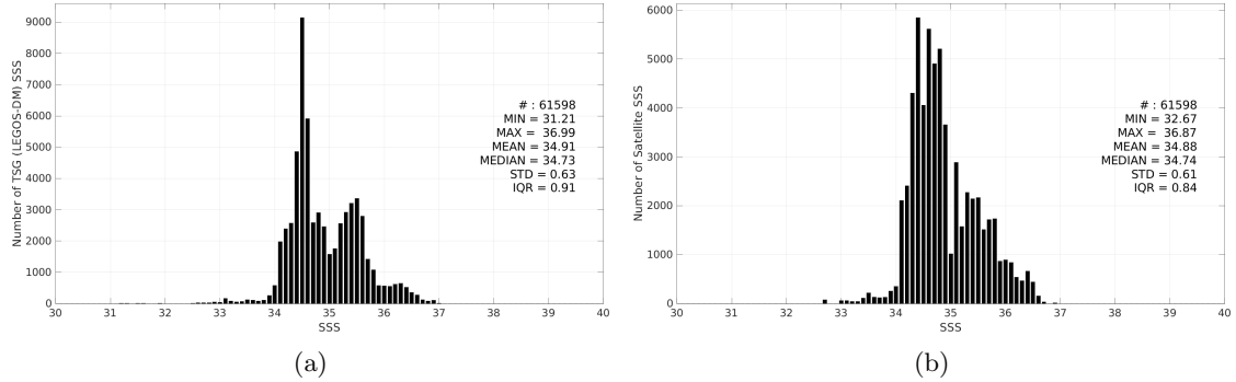
Figure 3: Histograms of SSS from TSG (LEGOS-DM) (a) and Aquarius SSS L3 OR v5 - Monthly - Rain mask (NASA-GSFC) (b) considering all match-up pairs per bins of 0.1 over the Indian Ocean Pi-MEP region and for the full satellite product period.
