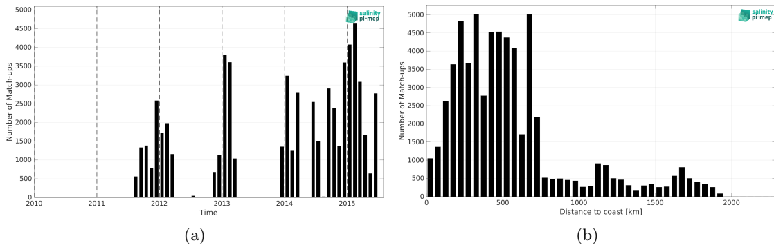
Figure 2: Number of match-ups between TSG (LEGOS-DM) and Aquarius SSS L3 OR v5 - Monthly - Rain mask (NASA-GSFC) SSS as a function of time (a) and as function of the distance to coast (b) over the Indian Ocean Pi-MEP region and for the full satellite product period.
