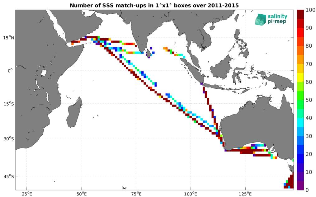
Figure 4: Number of SSS match-ups between TSG (LEGOS-DM) SSS and the Aquarius SSS L3 OR v5 - Monthly - Rain mask (NASA-GSFC) SSS product for the Indian Ocean Pi-MEP region over 1^{\circ} \times 1^{\circ} boxes and for the full satellite product period.
