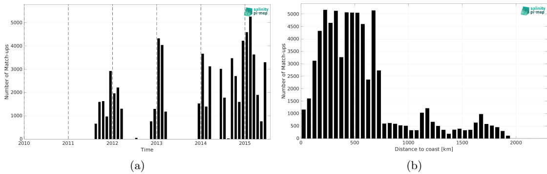
Figure 1: Number of match-ups between TSG (LEGOS-DM) and Aquarius SSS L3 OR v5 - Monthly - Rain mask (NASA-GSFC) SSS as a function of time (a) and as function of the distance to coast (b) over the Indian Ocean Pi-MEP region and for the full satellite product period.
