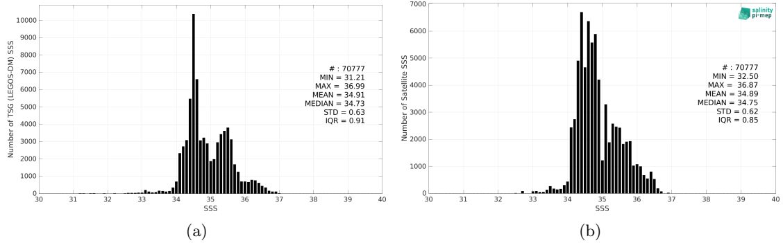
Figure 2: Histograms of SSS from TSG (LEGOS-DM) (a) and Aquarius SSS L3 OR v5 - Monthly - Rain mask (NASA-GSFC) (b) considering all match-up pairs per bins of 0.1 over the Indian Ocean Pi-MEP region and for the full satellite product period.
