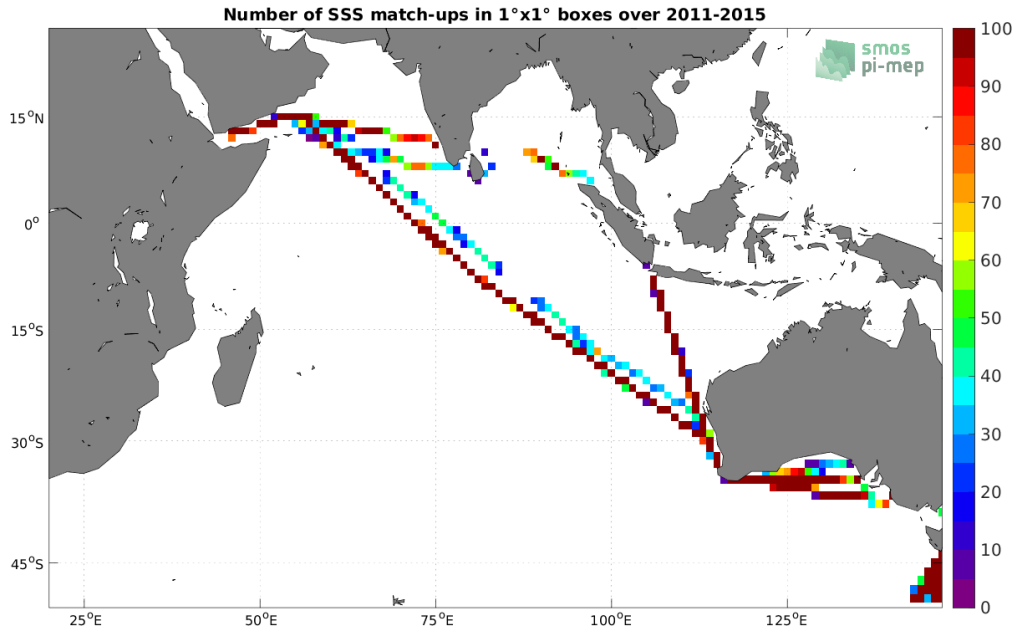
Figure 4: Number of SSS match-ups between TSG (LEGOS-DM) SSS and the Aquarius SSS L3 OR v5 - Monthly - Rain mask (NASA-GSFC) SSS product for the Indian Ocean Pi-MEP region over 1^\circ \times 1^\circ boxes and for the full satellite product period.
