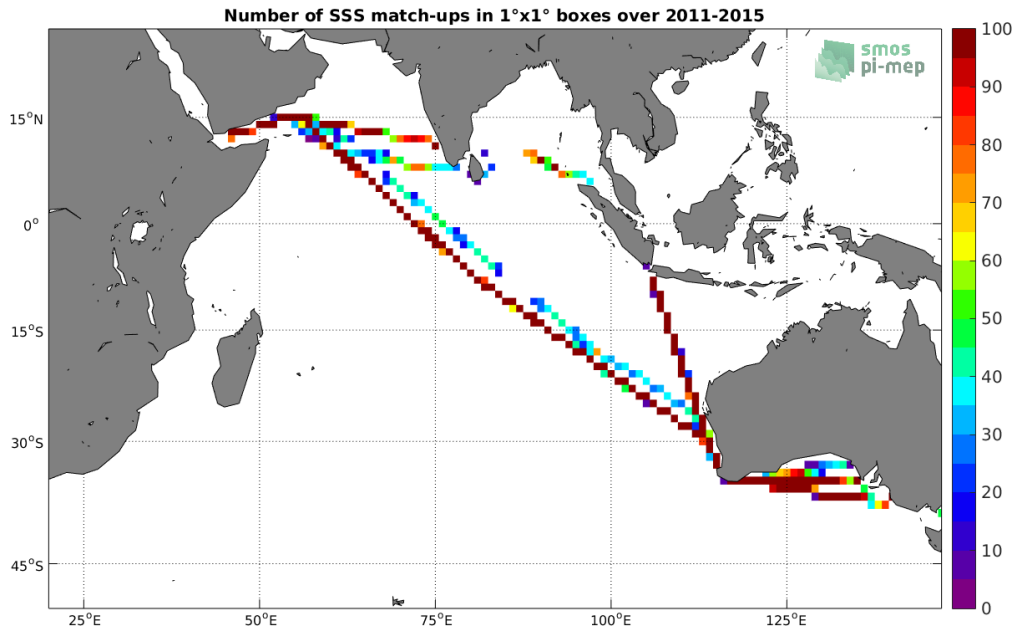
Figure 4: Number of SSS match-ups between TSG-LEGOS-DM SSS and the Aquarius-L3-OR-V5-MONTHLY-RAIN-MASK-1DEG SSS product for the Indian Ocean Pi-MEP region over 1^\circ \times 1^\circ boxes and for the full satellite product period.
