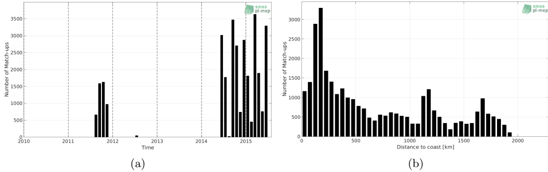
Figure 1: Number of match-ups between TSG-LEGOS-DM and Aquarius-L3-OR-V5-MONTHLY-RAIN-MASK-1DEG SSS as a function of time (a) and as function of the distance to coast (b) over the Indian Ocean Pi-MEP region and for the full satellite product period.
