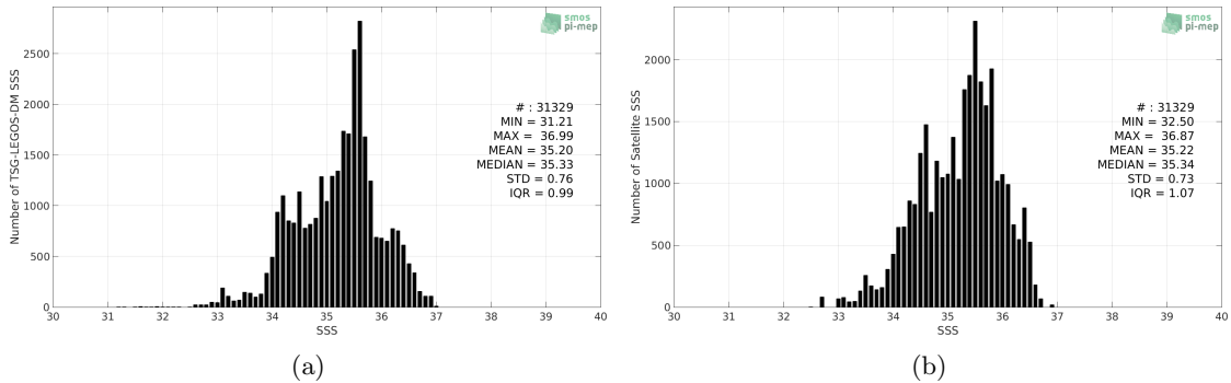
Figure 2: Histograms of SSS from TSG-LEGOS-DM (a) and Aquarius-L3-OR-V5-MONTHLY-RAIN-MASK-1DEG (b) considering all match-up pairs per bins of 0.1 over the Indian Ocean Pi-MEP region and for the full satellite product period.
