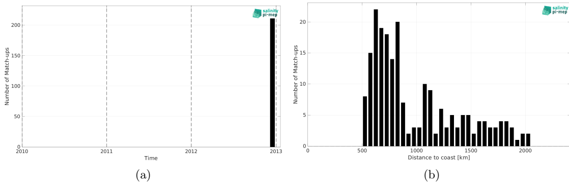
Figure 2: Number of match-ups between TSG (GOSUD-Sailing-ship) and Aquarius SSS L3 OR v5 - Monthly - Rain mask (NASA-GSFC) SSS as a function of time (a) and as function of the distance to coast (b) over the Indian Ocean Pi-MEP region and for the full satellite product period.
