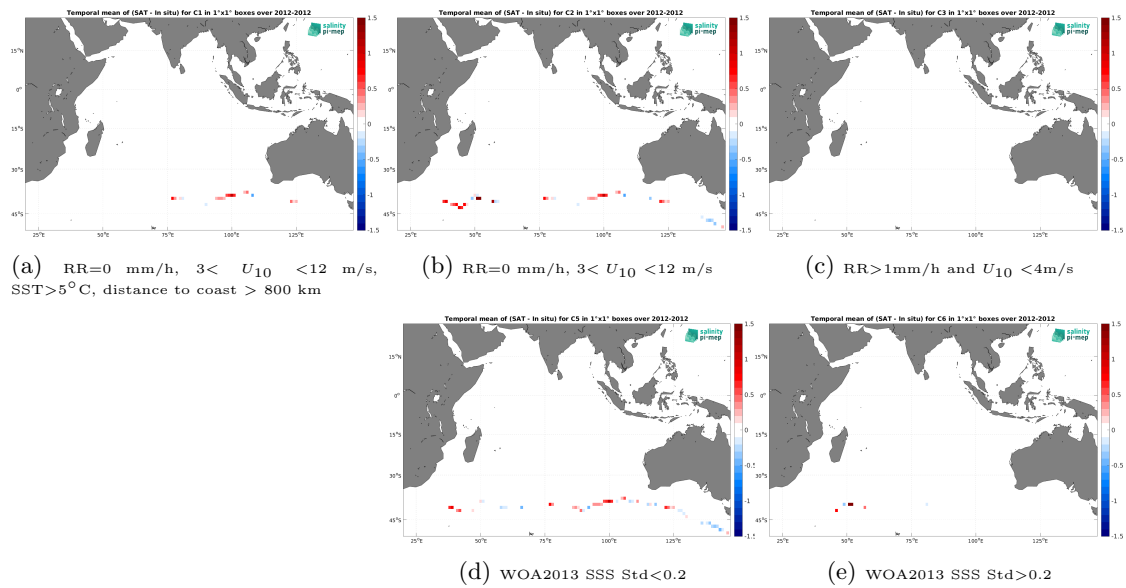
Figure 14: Temporal mean gridded over spatial boxes of size 1^\circ \times 1^\circ of \Delta SSS (Aquarius SSS L3 OR v5 - Monthly - Rain mask (NASA-GSFC) - TSG (GOSUD-Sailing-ship)) for 5 different subdatasets corresponding to:RR=0 mm/h, 3 < U_{10} < 12 m/s, SST >5^\circ C, distance to coast > 800 km (a), RR=0 mm/h, 3 < U_{10} < 12 m/s (b), RR >1 mm/h and U_{10} < 4 m/s (c), WOA2013 SSS Std <0.2 (d), WOA2013 SSS Std >0.2 (e).
