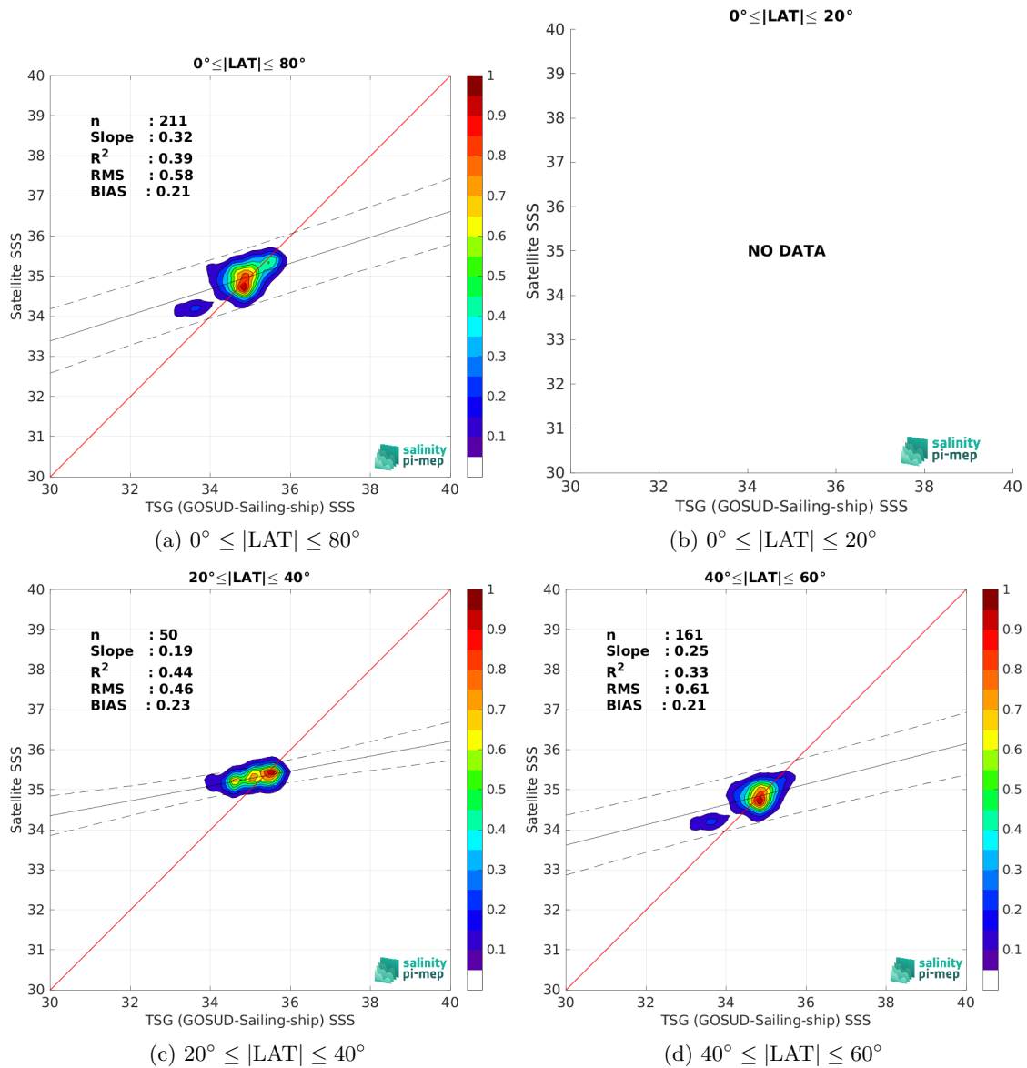
Figure 10: Contour maps of the concentration of Aquarius SSS L3 OR v5 - Monthly - Rain mask (NASA-GSFC) SSS (y-axis) versus TSG (GOSUD-Sailing-ship) SSS (x-axis) at match-up pairs for different latitude bands. For each plot, the red line shows x=y . The black thin and dashed lines indicate a linear fit through the data cloud and the \pm 95\% confidence levels, respectively. The number match-up pairs n , the slope and R^2 coefficient of the linear fit, the root mean square (RMS) and the mean bias between satellite and in situ data are indicated for each latitude band in each plots.
