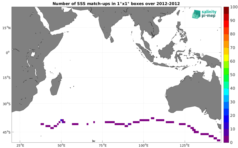
Figure 5: Number of SSS match-ups between TSG (GOSUD-Sailing-ship) SSS and the Aquarius SSS L3 OR v5 - Monthly - Rain mask (NASA-GSFC) SSS product for the Indian Ocean Pi-MEP region over 1^\circ \times 1^\circ boxes and for the full satellite product period.
