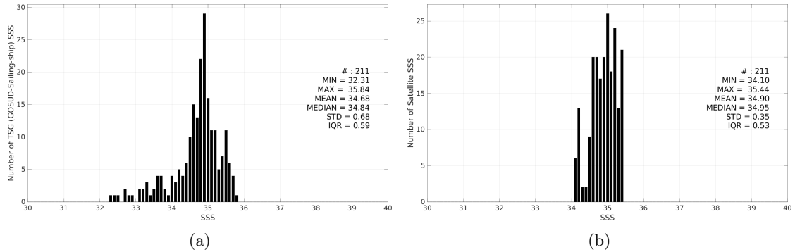
Figure 3: Histograms of SSS from TSG (GOSUD-Sailing-ship) (a) and Aquarius SSS L3 OR v5 - Monthly - Rain mask (NASA-GSFC) (b) considering all match-up pairs per bins of 0.1 over the Indian Ocean Pi-MEP region and for the full satellite product period.
