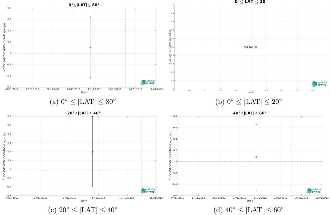
Figure 11: Monthly median (red curves) of \Delta SSS (Satellite - TSG (GOSUD-Sailing-ship)) and \pm 1 Std (black vertical thick bars) as function of time for all the collected Pi-MEP match-up pairs estimated over the Indian Ocean Pi-MEP region and for the full satellite product period are shown for different latitude bands: (a) 80^\circ\text{S}-80^\circ\text{N} , (b) 20^\circ\text{S}-20^\circ\text{N} , (c) 40^\circ\text{S}-20^\circ\text{S} and 20^\circ\text{N}-40^\circ\text{N} and (d) 60^\circ\text{S}-40^\circ\text{S} and 40^\circ\text{N}-60^\circ\text{N} .
