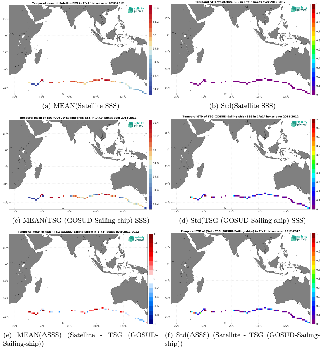
Figure 7: Temporal mean (left) and Std (right) of SSS from Aquarius SSS L3 OR v5 - Monthly - Rain mask (NASA-GSFC) (top), TSG (GOSUD-Sailing-ship) (middle), and of \Delta SSS (Satellite - TSG (GOSUD-Sailing-ship)). Only match-up pairs are used to generate these maps.
