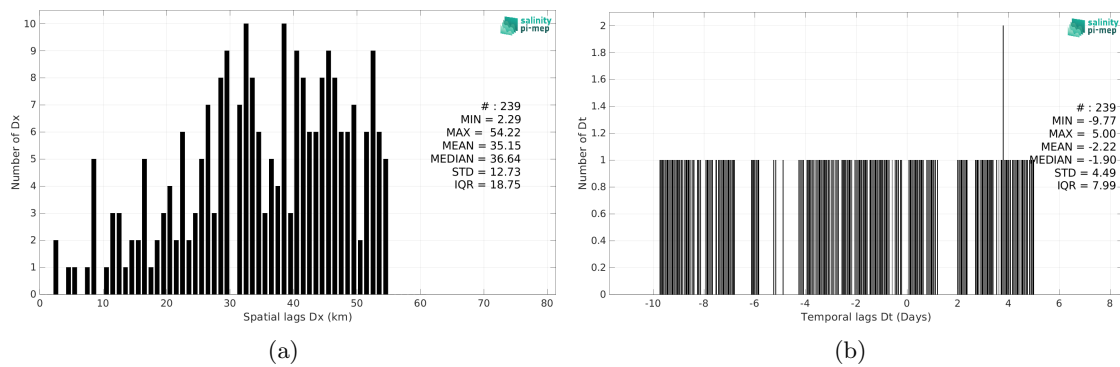
Figure 5: Histograms of the spatial (a) and temporal (b) lags between the location/time of the TSG (GOSUD-Sailing-ship) measurement and the date of the corresponding Aquarius SSS L3 OR v5 - Monthly - Rain mask (NASA-GSFC) SSS pixel.
