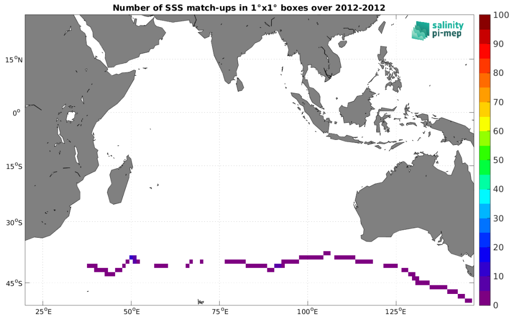
Figure 4: Number of SSS match-ups between TSG (GOSUD-Sailing-ship) SSS and the Aquarius SSS L3 OR v5 - Monthly - Rain mask (NASA-GSFC) SSS product for the Indian Ocean Pi-MEP region over 1^\circ \times 1^\circ boxes and for the full satellite product period.
