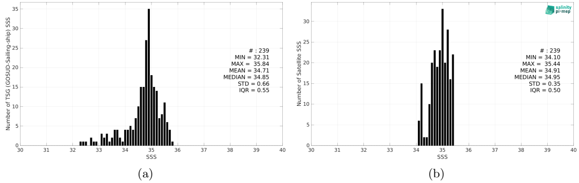
Figure 2: Histograms of SSS from TSG (GOSUD-Sailing-ship) (a) and Aquarius SSS L3 OR v5 - Monthly - Rain mask (NASA-GSFC) (b) considering all match-up pairs per bins of 0.1 over the Indian Ocean Pi-MEP region and for the full satellite product period.
