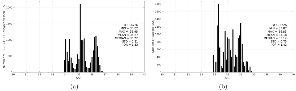
Figure 3: Histograms of SSS from TSG (GOSUD-Research-vessel) (a) and Aquarius SSS L3 OR v5 - Monthly - Rain mask (NASA-GSFC) (b) considering all match-up pairs per bins of 0.1 over the Indian Ocean Pi-MEP region and for the full satellite product period.
