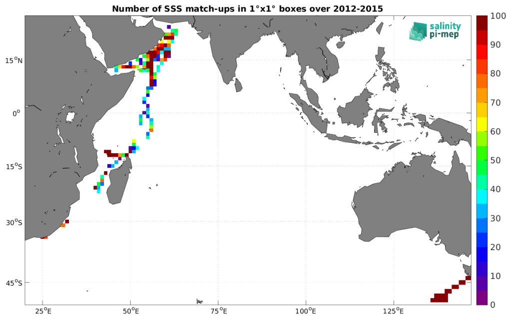
Figure 5: Number of SSS match-ups between TSG (GOSUD-Research-vessel) SSS and the Aquarius SSS L3 OR v5 - Monthly - Rain mask (NASA-GSFC) SSS product for the Indian Ocean Pi-MEP region over 1^{\circ} \times 1^{\circ} boxes and for the full satellite product period.
