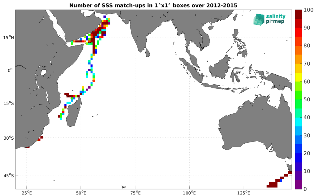
Figure 4: Number of SSS match-ups between TSG (GOSUD-Research-vessel) SSS and the Aquarius SSS L3 OR v5 - Monthly - Rain mask (NASA-GSFC) SSS product for the Indian Ocean Pi-MEP region over 1^\circ \times 1^\circ boxes and for the full satellite product period.
