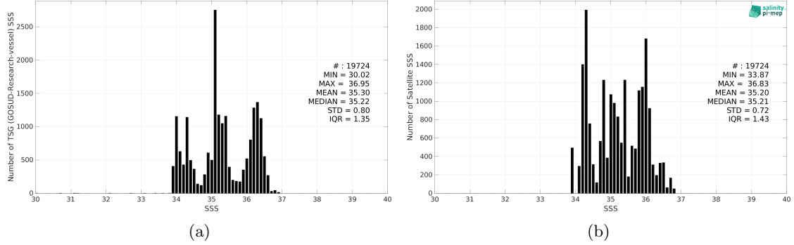
Figure 2: Histograms of SSS from TSG (GOSUD-Research-vessel) (a) and Aquarius SSS L3 OR v5 - Monthly - Rain mask (NASA-GSFC) (b) considering all match-up pairs per bins of 0.1 over the Indian Ocean Pi-MEP region and for the full satellite product period.
