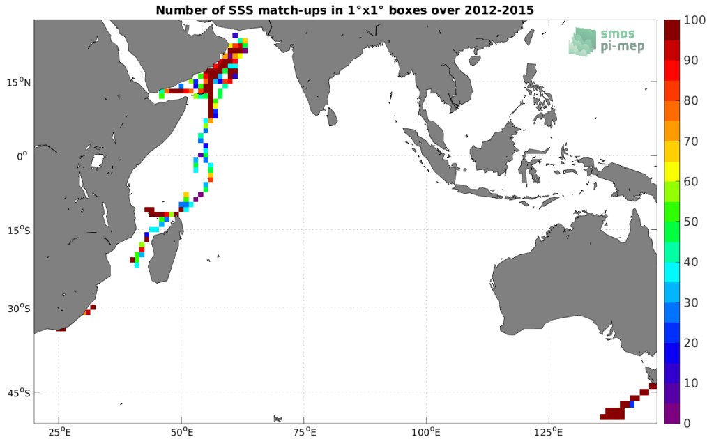
Figure 4: Number of SSS match-ups between TSG (GOSUD-Research-vessel) SSS and the Aquarius SSS L3 OR v5 - Monthly - Rain mask (NASA-GSFC) SSS product for the Indian Ocean Pi-MEP region over 1^{\circ} \times 1^{\circ} boxes and for the full satellite product period.
