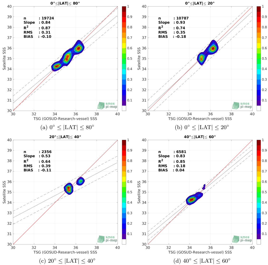
Figure 9: Contour maps of the concentration of Aquarius SSS L3 OR v5 - Monthly - Rain mask (NASA-GSFC) SSS ( y -axis) versus TSG (GOSUD-Research-vessel) SSS ( x -axis) at match-up pairs for different latitude bands. For each plot, the red line shows x=y . The black thin and dashed lines indicate a linear fit through the data cloud and the \pm 95\% confidence levels, respectively. The number match-up pairs n , the slope and R^2 coefficient of the linear fit, the root mean square (RMS) and the mean bias between satellite and in situ data are indicated for each latitude band in each plots.
