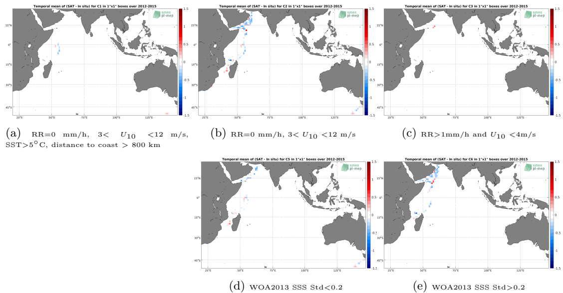
Figure 12: Temporal mean gridded over spatial boxes of size 1^\circ \times 1^\circ of \Delta\text{SSS} (Aquarius SSS L3 OR v5 - Monthly - Rain mask (NASA-GSFC) - TSG (GOSUD-Research-vessel)) for 5 different subdatasets corresponding to: RR=0 mm/h, 3 < U_{10} < 12 m/s, SST > 5°C, distance to coast > 800 km (a), RR=0 mm/h, 3 < U_{10} < 12 m/s (b), RR > 1mm/h and U_{10} < 4 m/s (c), WOA2013 SSS Std < 0.2 (d), WOA2013 SSS Std > 0.2 (e).
