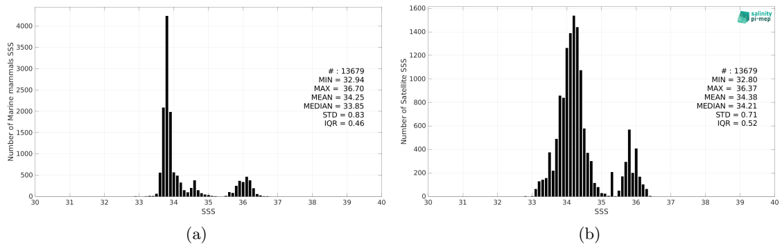
Figure 2: Histograms of SSS from Marine mammals (a) and Aquarius SSS L3 OR v5 - Monthly - Rain mask (NASA-GSFC) (b) considering all match-up pairs per bins of 0.1 over the Indian Ocean Pi-MEP region and for the full satellite product period.
