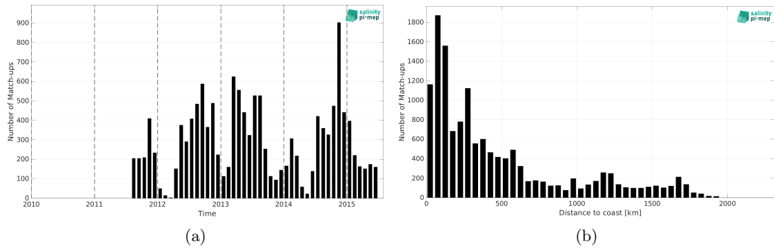
Figure 1: Number of match-ups between Marine mammals and Aquarius SSS L3 OR v5 - Monthly - Rain mask (NASA-GSFC) SSS as a function of time (a) and as function of the distance to coast (b) over the Indian Ocean Pi-MEP region and for the full satellite product period.
