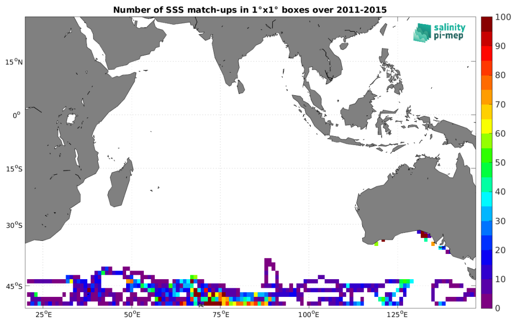
Figure 4: Number of SSS match-ups between Marine mammals SSS and the Aquarius SSS L3 OR v5 - Monthly - Rain mask (NASA-GSFC) SSS product for the Indian Ocean Pi-MEP region over 1^\circ \times 1^\circ boxes and for the full satellite product period.
