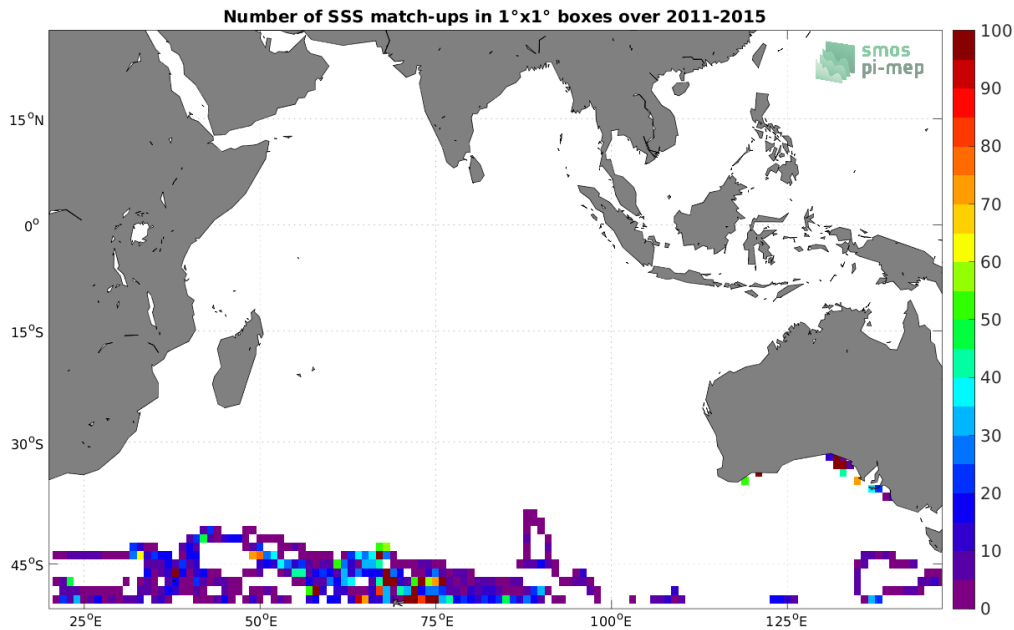
Figure 4: Number of SSS match-ups between Marine mammals SSS and the Aquarius SSS L3 OR v5 - Monthly - Rain mask (NASA-GSFC) SSS product for the Indian Ocean Pi-MEP region over 1^\circ \times 1^\circ boxes and for the full satellite product period.
