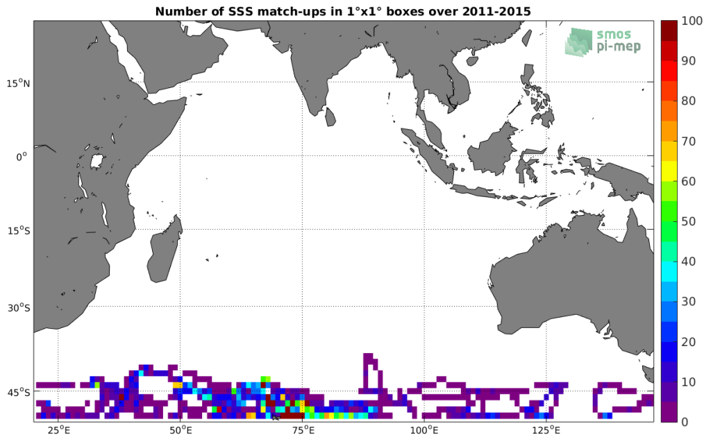
Figure 4: Number of SSS match-ups between Sea mammals SSS and the Aquarius-L3-OR-V5-MONTHLY-RAIN-MASK-1DEG SSS product for the Indian Ocean Pi-MEP region over 1°x1° boxes and for the full satellite product period.
