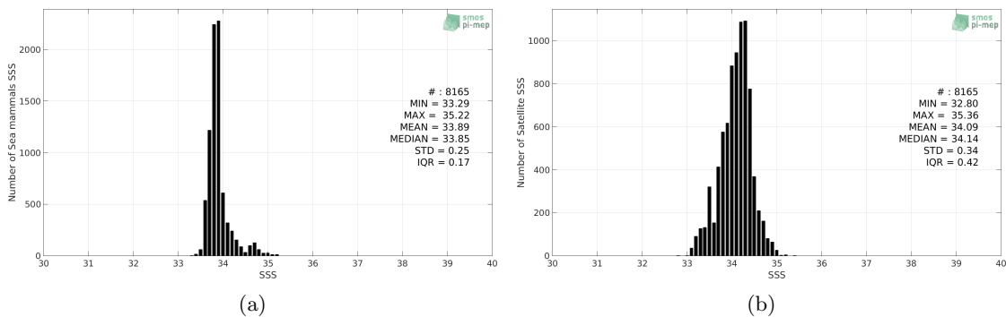
Figure 2: Histograms of SSS from Sea mammals (a) and Aquarius-L3-OR-V5-MONTHLY-RAIN-MASK-1DEG (b) considering all match-up pairs per bins of 0.1 over the Indian Ocean Pi-MEP region and for the full satellite product period.
