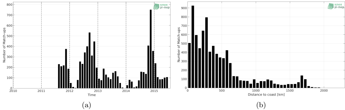
Figure 1: Number of match-ups between Sea mammals and Aquarius-L3-OR-V5-MONTHLY-RAIN-MASK-1DEG SSS as a function of time (a) and as function of the distance to coast (b) over the Indian Ocean Pi-MEP region and for the full satellite product period.
