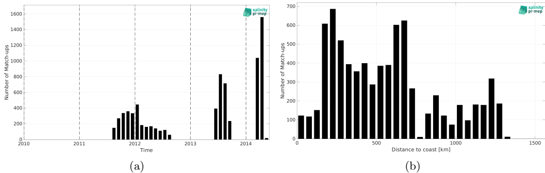
Figure 2: Number of match-ups between Surface drifters and Aquarius SSS L3 OR v5 - Monthly - Rain mask (NASA-GSFC) SSS as a function of time (a) and as function of the distance to coast (b) over the Indian Ocean Pi-MEP region and for the full satellite product period.
