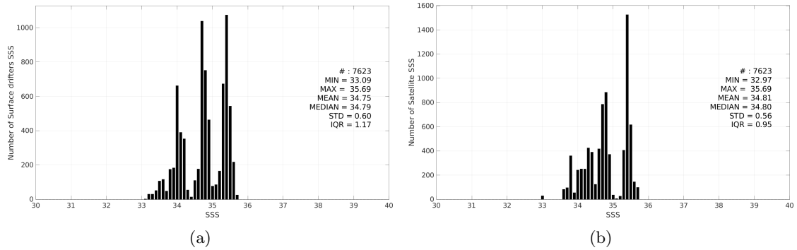
Figure 3: Histograms of SSS from Surface drifters (a) and Aquarius SSS L3 OR v5 - Monthly - Rain mask (NASA-GSFC) (b) considering all match-up pairs per bins of 0.1 over the Indian Ocean Pi-MEP region and for the full satellite product period.
