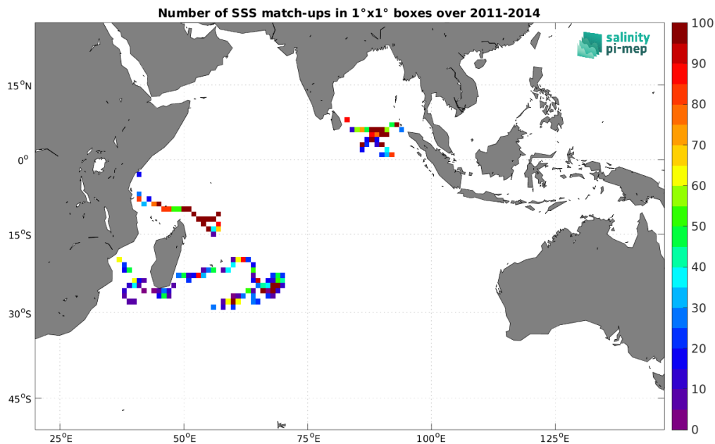
Figure 4: Number of SSS match-ups between Surface drifters SSS and the Aquarius SSS L3 OR v5 - Monthly - Rain mask (NASA-GSFC) SSS product for the Indian Ocean Pi-MEP region over 1^\circ \times 1^\circ boxes and for the full satellite product period.
