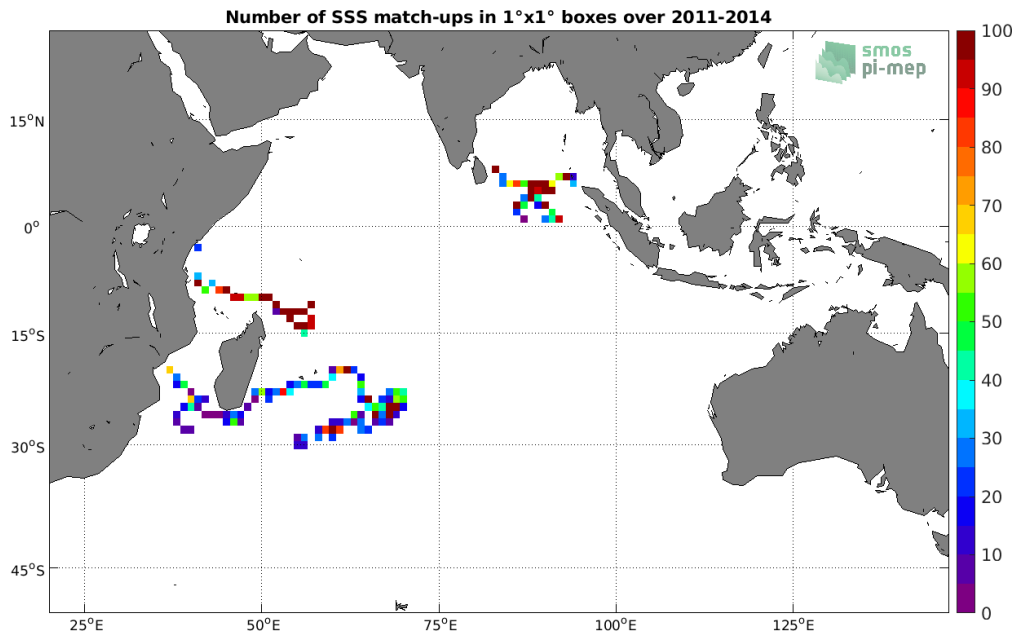
Figure 3: Number of SSS match-ups between Surface drifters SSS and the Aquarius SSS L3 OR v5 - Monthly - Rain mask (NASA-GSFC) SSS product for the Indian Ocean Pi-MEP region over 1^\circ \times 1^\circ boxes and for the full satellite product period.
