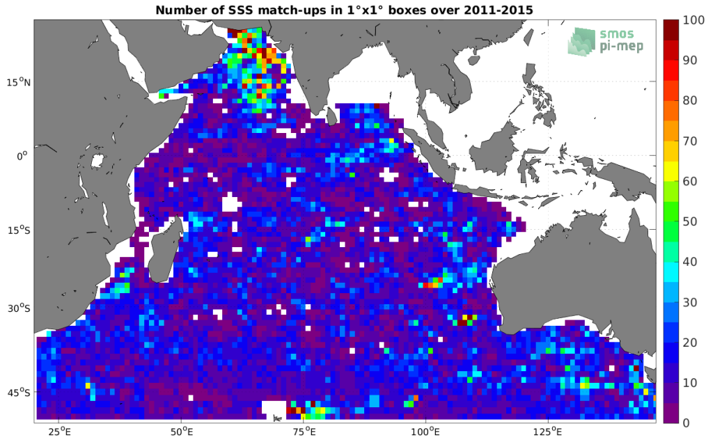
Figure 4: Number of SSS match-ups between Argo SSS and the Aquarius SSS L3 OR v5 - Monthly - Rain mask (NASA-GSFC) SSS product for the Indian Ocean Pi-MEP region over 1^\circ \times 1^\circ boxes and for the full satellite product period.
