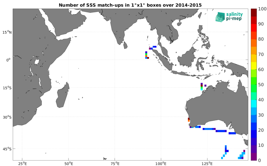
Figure 5: Number of SSS match-ups between TSG (SAMOS) SSS and the Aquarius SSS L3 CAP v5 - 7-Day running (JPL) SSS product for the Indian Ocean Pi-MEP region over 1^\circ \times 1^\circ boxes and for the full satellite product period.
