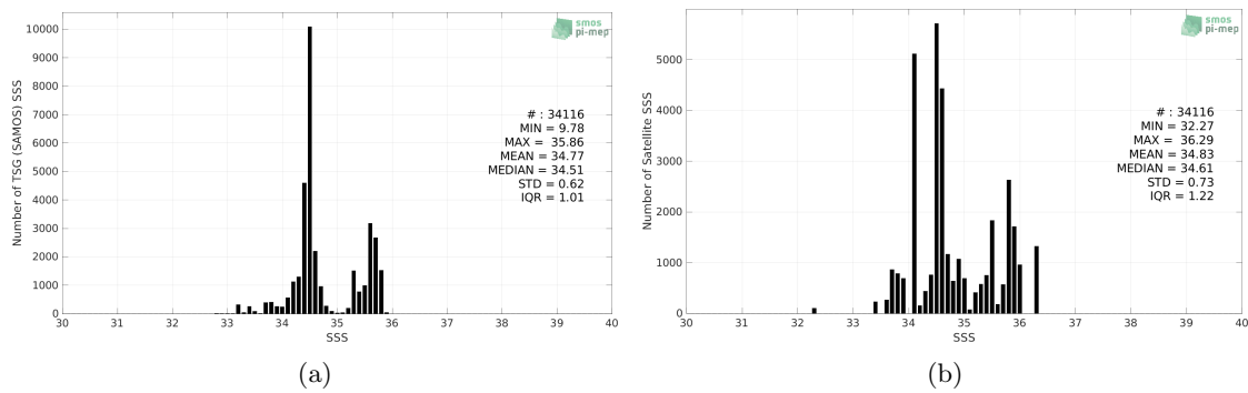
Figure 2: Histograms of SSS from TSG (SAMOS) (a) and Aquarius SSS L3 CAP v5 - 7-Day running (JPL) (b) considering all match-up pairs per bins of 0.1 over the Indian Ocean Pi-MEP region and for the full satellite product period.
