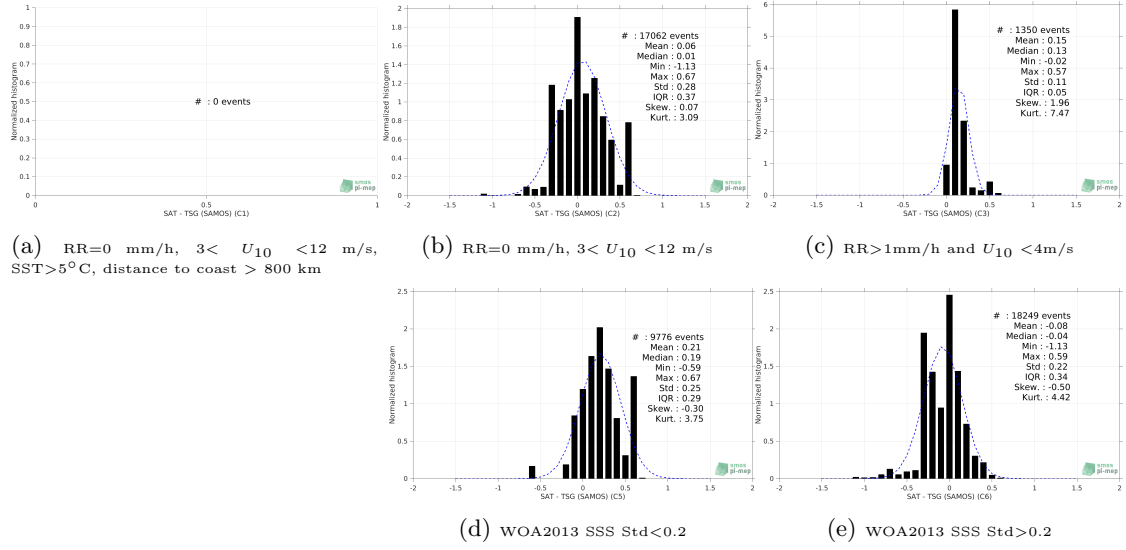
Figure 13: Normalized histogram of \Delta\text{SSS} (Aquarius SSS L3 CAP v5 - 7-Day running (JPL) - TSG (SAMOS)) for 5 different subdatasets corresponding to: RR=0 mm/h, 3 < U_{10} < 12 m/s, SST > 5^\circ\text{C} , distance to coast > 800 km (a), RR=0 mm/h, 3 < U_{10} < 12 m/s (b), RR > 1\text{mm/h} and U_{10} < 4\text{m/s} (c), WOA2013 SSS Std < 0.2 (d), WOA2013 SSS Std > 0.2 (e).
