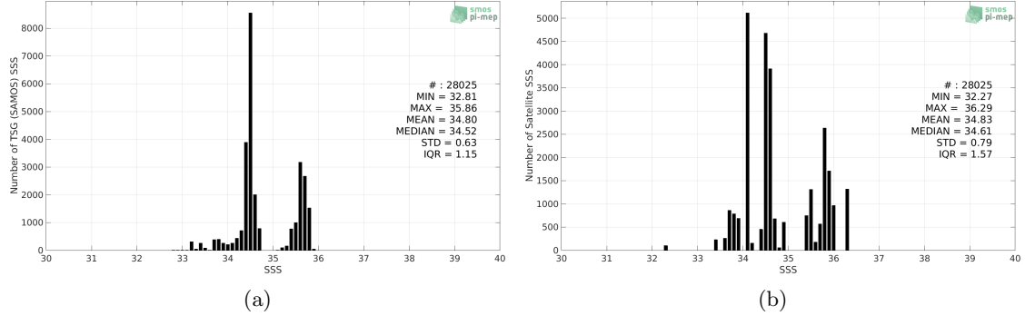
Figure 2: Histograms of SSS from TSG (SAMOS) (a) and Aquarius SSS L3 CAP v5 - 7-Day running (JPL) (b) considering all match-up pairs per bins of 0.1 over the Indian Ocean Pi-MEP region and for the full satellite product period.
