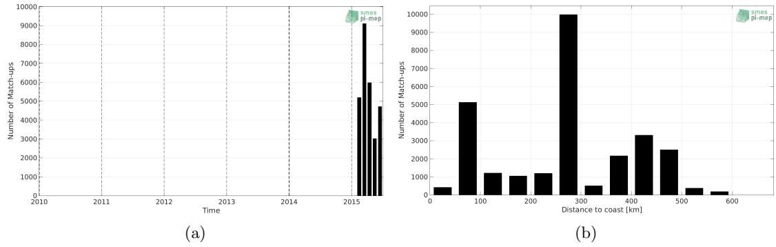
Figure 1: Number of match-ups between TSG (SAMOS) and Aquarius SSS L3 CAP v5 - 7-Day running (JPL) SSS as a function of time (a) and as function of the distance to coast (b) over the Indian Ocean Pi-MEP region and for the full satellite product period.
