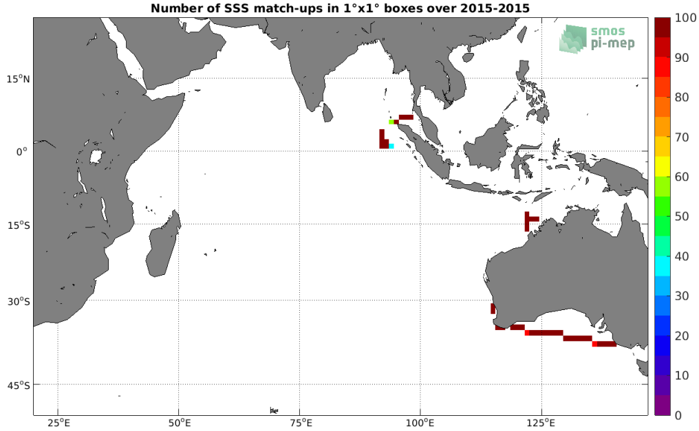
Figure 4: Number of SSS match-ups between TSG (SAMOS) SSS and the Aquarius SSS L3 CAP v5 - 7-Day running (JPL) SSS product for the Indian Ocean Pi-MEP region over 1^\circ \times 1^\circ boxes and for the full satellite product period.
