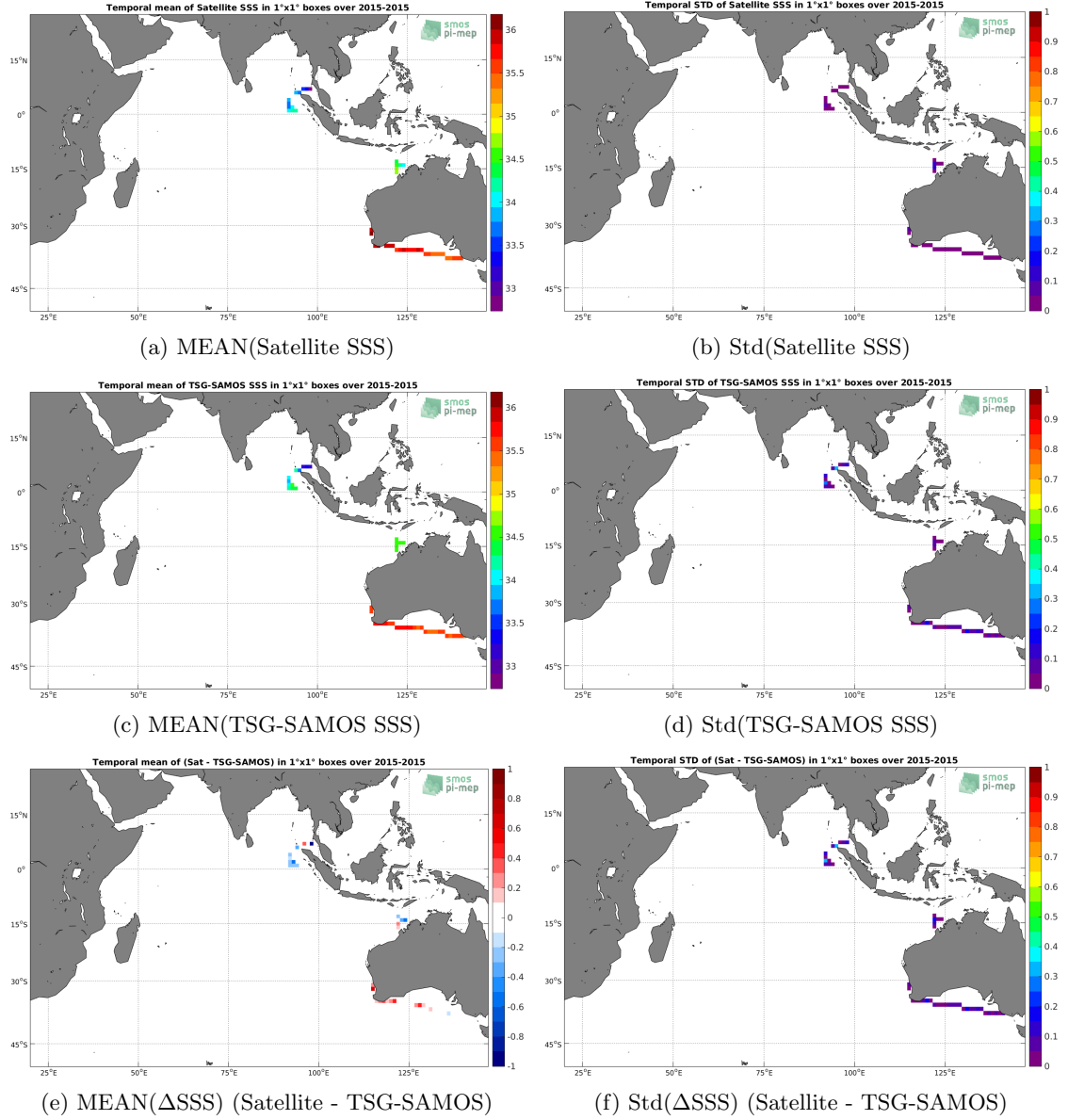
Figure 6: Temporal mean (left) and Std (right) of SSS from Aquarius-L3-JPL-V5-7DAY-RUNNING (top), TSG-SAMOS (middle), and of \Delta SSS (Satellite - TSG-SAMOS). Only match-up pairs are used to generate these maps.
