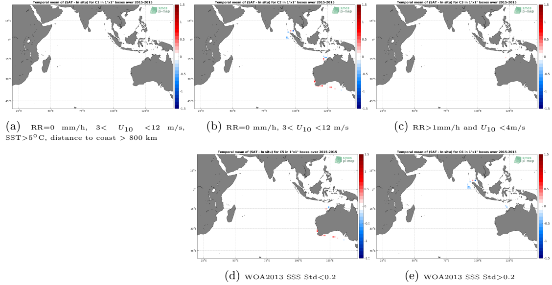
Figure 12: Temporal mean gridded over spatial boxes of size 1^\circ \times 1^\circ of \Delta SSS (Aquarius-L3-JPL-V5-7DAY-RUNNING - TSG-SAMOS) for 5 different subdatasets corresponding to: RR=0 mm/h, 3 < U_{10} < 12 m/s, SST > 5^\circ C , distance to coast > 800 km (a), RR=0 mm/h, 3 < U_{10} < 12 m/s (b), RR > 1 mm/h and U_{10} < 4 m/s (c), WOA2013 SSS Std < 0.2 (d), WOA2013 SSS Std > 0.2 (e).
