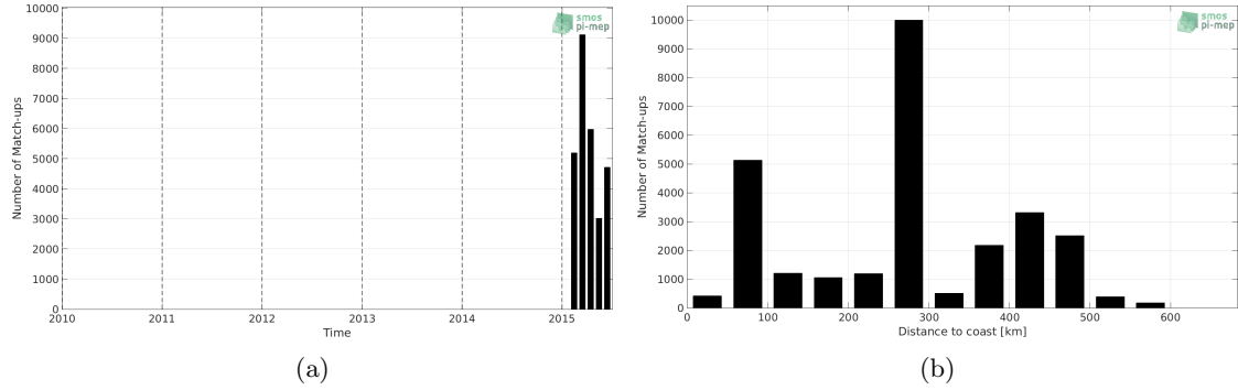
Figure 1: Number of match-ups between TSG-SAMOS and Aquarius-L3-JPL-V5-7DAY-RUNNING SSS as a function of time (a) and as function of the distance to coast (b) over the Indian Ocean Pi-MEP region and for the full satellite product period.
