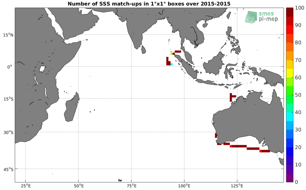
Figure 4: Number of SSS match-ups between TSG-SAMOS SSS and the Aquarius-L3-JPL-V5-7DAY-RUNNING SSS product for the Indian Ocean Pi-MEP region over 1°x1° boxes and for the full satellite product period.
