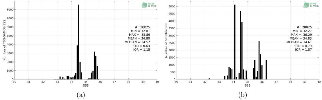
Figure 2: Histograms of SSS from TSG-SAMOS (a) and Aquarius-L3-JPL-V5-7DAY-RUNNING (b) considering all match-up pairs per bins of 0.1 over the Indian Ocean Pi-MEP region and for the full satellite product period.
