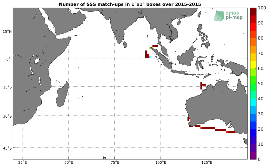
Figure 4: Number of SSS match-ups between TSG-SAMOS SSS and the Aquarius-L3-JPL-V5-7DAY-RUNNING SSS product for the Indian Ocean Pi-MEP region over 1^\circ \times 1^\circ boxes and for the full satellite product period.
