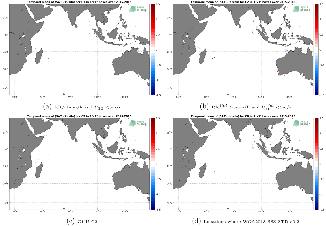
Figure 12: Temporal mean gridded over spatial boxes of size 1^\circ \times 1^\circ of \Delta SSS (Aquarius-L3-JPL-V5-7DAY-RUNNING - TSG-SAMOS) for 4 different subdatasets corresponding to: RR > 1\text{mm/h} and U_{10} < 5\text{m/s} (a), RR^{10d} > 5\text{mm/h} and U_{10}^{10d} < 5\text{m/s} (b), C1 U C2 (c), Locations where WOA2013 SSS STD > 0.2 (d).
