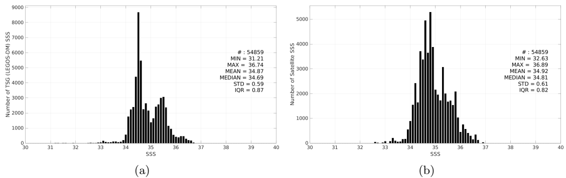
Figure 3: Histograms of SSS from TSG (LEGOS-DM) (a) and Aquarius SSS L3 CAP v5 - 7-Day running (JPL) (b) considering all match-up pairs per bins of 0.1 over the Indian Ocean Pi-MEP region and for the full satellite product period.
