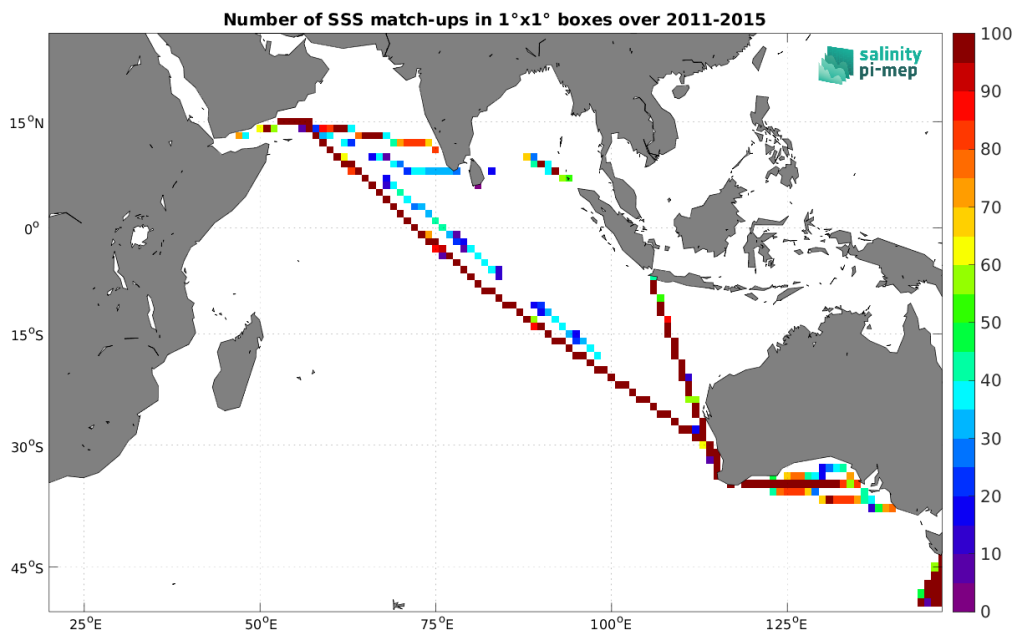
Figure 5: Number of SSS match-ups between TSG (LEGOS-DM) SSS and the Aquarius SSS L3 CAP v5 - 7-Day running (JPL) SSS product for the Indian Ocean Pi-MEP region over 1^\circ \times 1^\circ boxes and for the full satellite product period.
