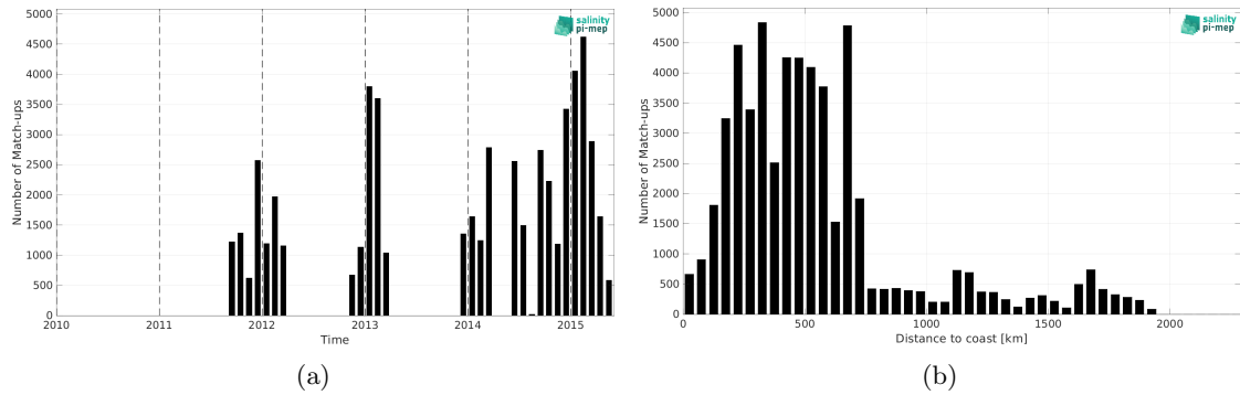
Figure 2: Number of match-ups between TSG (LEGOS-DM) and Aquarius SSS L3 CAP v5 - 7-Day running (JPL) SSS as a function of time (a) and as function of the distance to coast (b) over the Indian Ocean Pi-MEP region and for the full satellite product period.
