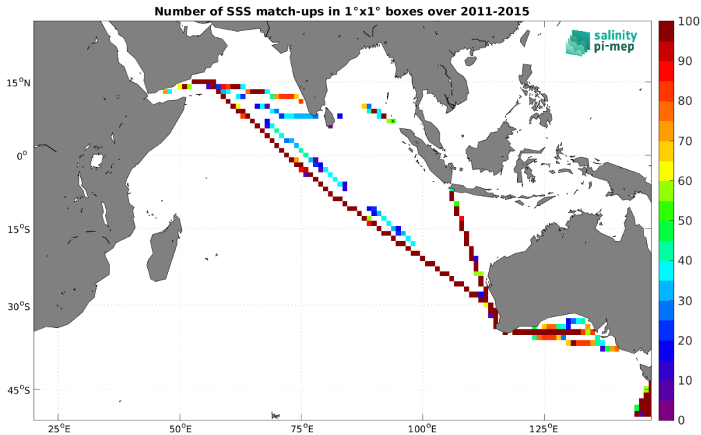
Figure 5: Number of SSS match-ups between TSG (LEGOS-DM) SSS and the Aquarius SSS L3 CAP v5 - 7-Day running (JPL) SSS product for the Indian Ocean Pi-MEP region over 1^\circ \times 1^\circ boxes and for the full satellite product period.
