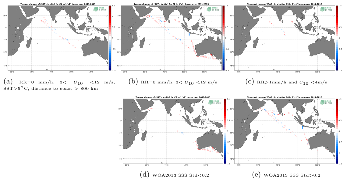
Figure 12: Temporal mean gridded over spatial boxes of size 1^\circ \times 1^\circ of \Delta\text{SSS} (Aquarius SSS L3 CAP v5 - 7-Day running (JPL) - TSG (LEGOS-DM)) for 5 different subdatasets corresponding to:RR=0 mm/h, 3 < U_{10} < 12 m/s, SST >5^\circ\text{C} , distance to coast > 800 km (a), RR=0 mm/h, 3 < U_{10} < 12 m/s (b), RR >1 mm/h and U_{10} < 4 m/s (c), WOA2013 SSS Std <0.2 (d), WOA2013 SSS Std >0.2 (e).
