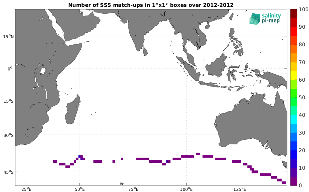
Figure 5: Number of SSS match-ups between TSG (GOSUD-Sailing-ship) SSS and the Aquarius SSS L3 CAP v5 - 7-Day running (JPL) SSS product for the Indian Ocean Pi-MEP region over 1^\circ \times 1^\circ boxes and for the full satellite product period.
