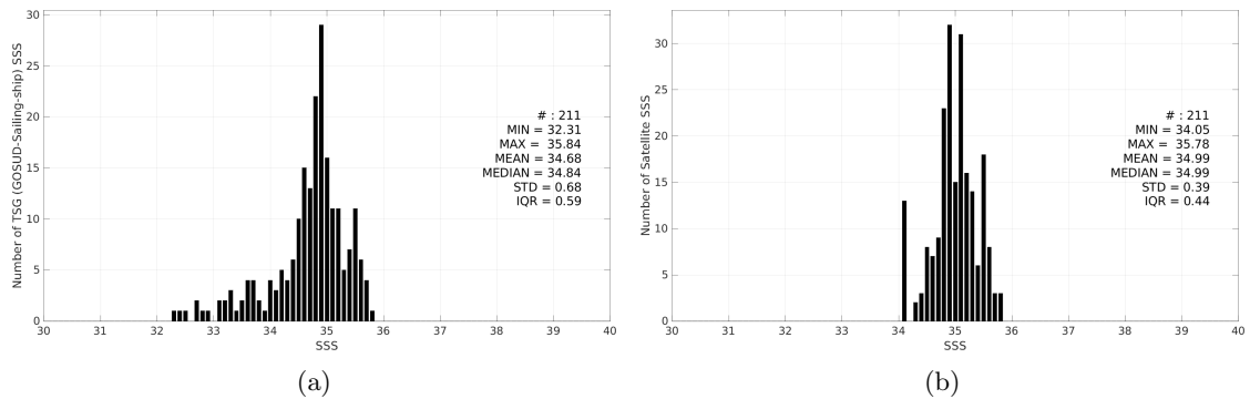
Figure 3: Histograms of SSS from TSG (GOSUD-Sailing-ship) (a) and Aquarius SSS L3 CAP v5 - 7-Day running (JPL) (b) considering all match-up pairs per bins of 0.1 over the Indian Ocean Pi-MEP region and for the full satellite product period.
