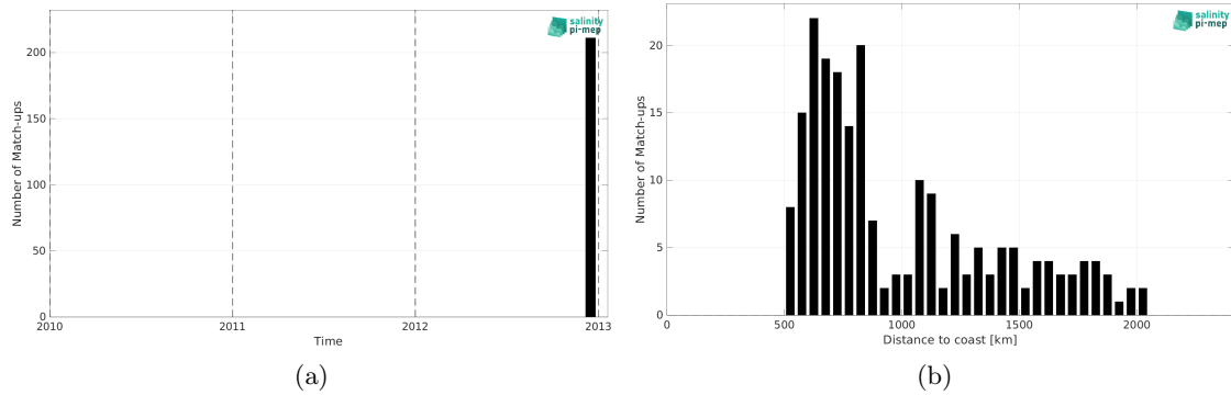
Figure 2: Number of match-ups between TSG (GOSUD-Sailing-ship) and Aquarius SSS L3 CAP v5 - 7-Day running (JPL) SSS as a function of time (a) and as function of the distance to coast (b) over the Indian Ocean Pi-MEP region and for the full satellite product period.
