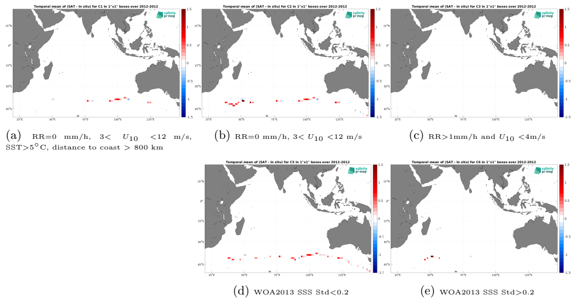
Figure 14: Temporal mean gridded over spatial boxes of size 1^\circ \times 1^\circ of \Delta\text{SSS} (Aquarius SSS L3 CAP v5 - 7-Day running (JPL) - TSG (GOSUD-Sailing-ship)) for 5 different subdatasets corresponding to:RR=0 mm/h, 3 < U_{10} < 12 m/s, SST >5^\circ\text{C} , distance to coast > 800 km (a), RR=0 mm/h, 3 < U_{10} < 12 m/s (b), RR >1 mm/h and U_{10} < 4 m/s (c), WOA2013 SSS Std <0.2 (d), WOA2013 SSS Std >0.2 (e).
