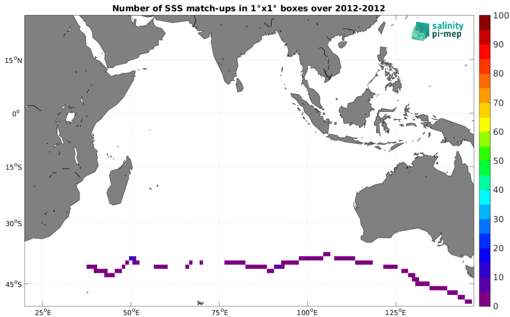
Figure 4: Number of SSS match-ups between TSG (GOSUD-Sailing-ship) SSS and the Aquarius SSS L3 CAP v5 - 7-Day running (JPL) SSS product for the Indian Ocean Pi-MEP region over 1°x1° boxes and for the full satellite product period.
