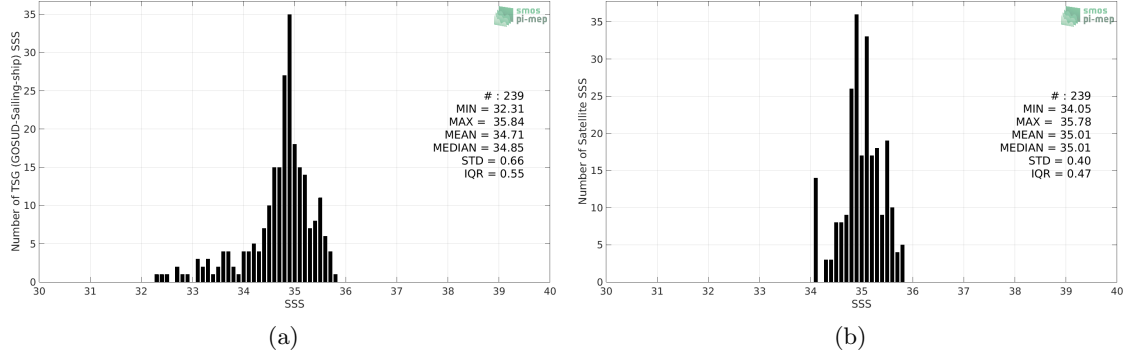
Figure 2: Histograms of SSS from TSG (GOSUD-Sailing-ship) (a) and Aquarius SSS L3 CAP v5 - 7-Day running (JPL) (b) considering all match-up pairs per bins of 0.1 over the Indian Ocean Pi-MEP region and for the full satellite product period.
