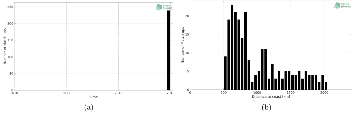
Figure 1: Number of match-ups between TSG (GOSUD-Sailing-ship) and Aquarius SSS L3 CAP v5 - 7-Day running (JPL) SSS as a function of time (a) and as function of the distance to coast (b) over the Indian Ocean Pi-MEP region and for the full satellite product period.
