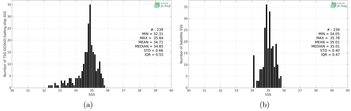
Figure 2: Histograms of SSS from TSG-GOSUD-Sailing-ship (a) and Aquarius-L3-JPL-V5-7DAY-RUNNING (b) considering all match-up pairs per bins of 0.1 over the Indian Ocean Pi-MEP region and for the full satellite product period.
