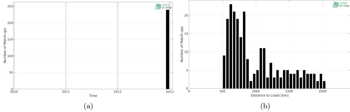
Figure 1: Number of match-ups between TSG-GOSUD-Sailing-ship and Aquarius-L3-JPL-V5-7DAY-RUNNING SSS as a function of time (a) and as function of the distance to coast (b) over the Indian Ocean Pi-MEP region and for the full satellite product period.
