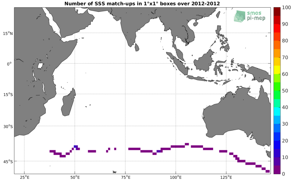
Figure 4: Number of SSS match-ups between TSG-GOSUD-Sailing-ship SSS and the Aquarius-L3-JPL-V5-7DAY-RUNNING SSS product for the Indian Ocean Pi-MEP region over 1^\circ \times 1^\circ boxes and for the full satellite product period.
