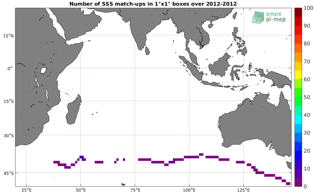
Figure 4: Number of SSS match-ups between TSG-GOSUD-Sailing-ship SSS and the Aquarius-L3-JPL-V5-7DAY-RUNNING SSS product for the Indian Ocean Pi-MEP region over 1°x1° boxes and for the full satellite product period.
