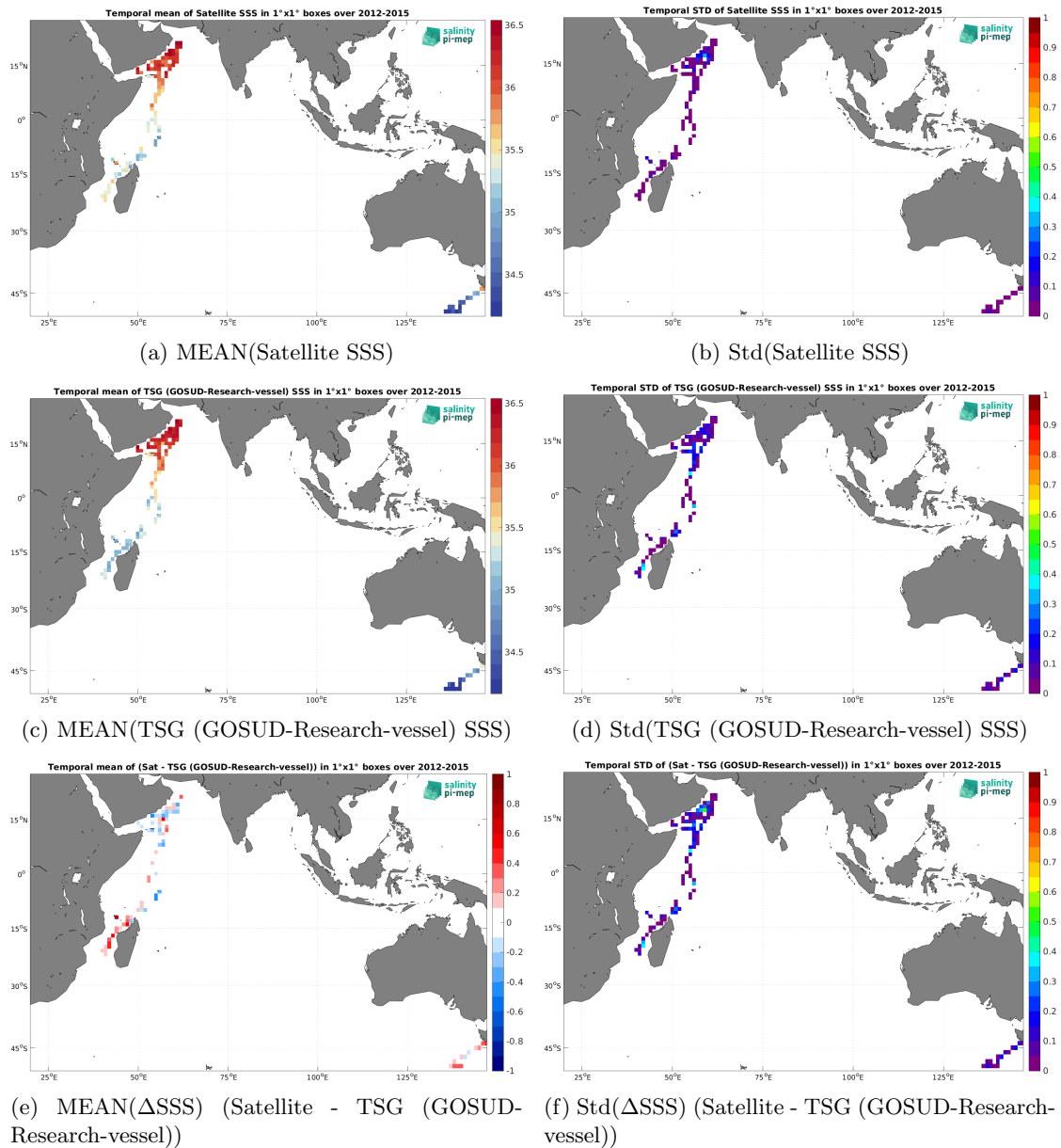
Figure 7: Temporal mean (left) and Std (right) of SSS from Aquarius SSS L3 CAP v5 - 7-Day running (JPL) (top), TSG (GOSUD-Research-vessel) (middle), and of \Delta SSS (Satellite - TSG (GOSUD-Research-vessel)). Only match-up pairs are used to generate these maps.
