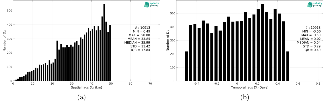
Figure 6: Histograms of the spatial (a) and temporal (b) lags between the location/time of the TSG (GOSUD-Research-vessel) measurement and the date of the corresponding Aquarius SSS L3 CAP v5 - 7-Day running (JPL) SSS pixel.
