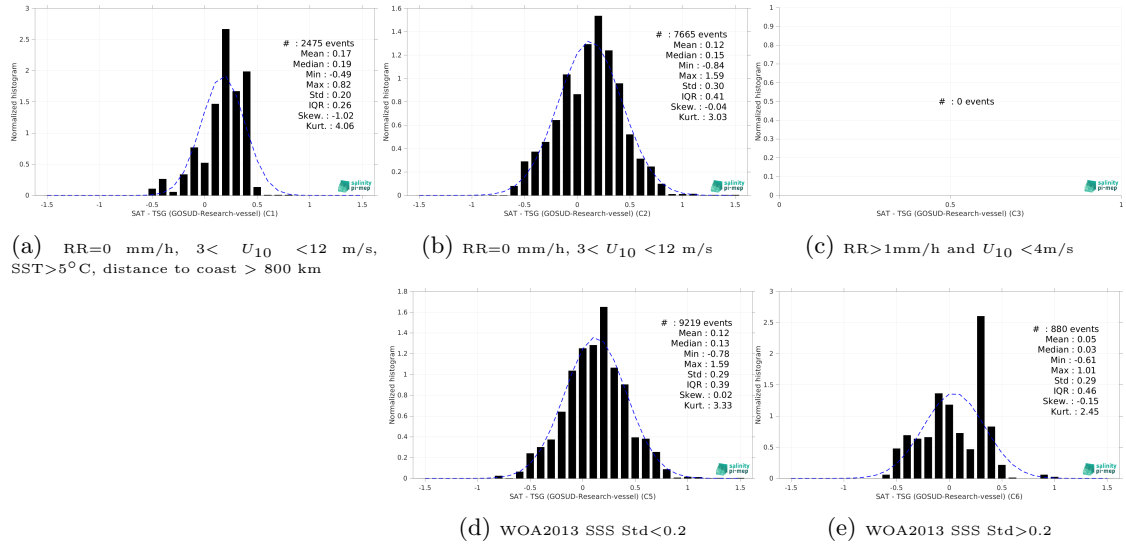
Figure 15: Normalized histogram of \Delta SSS (Aquarius SSS L3 CAP v5 - 7-Day running (JPL) - TSG (GOSUD-Research-vessel)) for 5 different subdatasets corresponding to: RR=0 mm/h, 3 < U_{10} < 12 m/s, SST > 5°C, distance to coast > 800 km (a), RR=0 mm/h, 3 < U_{10} < 12 m/s (b), RR > 1mm/h and U_{10} < 4 m/s (c), WOA2013 SSS Std < 0.2 (d), WOA2013 SSS Std > 0.2 (e).
