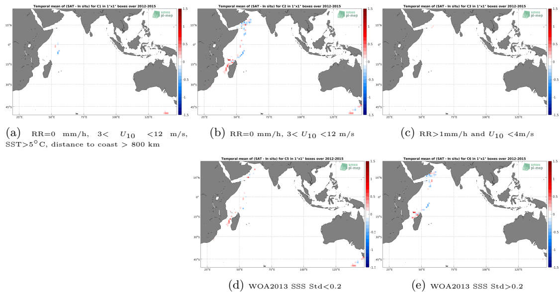
Figure 12: Temporal mean gridded over spatial boxes of size 1^\circ \times 1^\circ of \Delta\text{SSS} (Aquarius SSS L3 CAP v5 - 7-Day running (JPL) - TSG (GOSUD-Research-vessel)) for 5 different subdatasets corresponding to: RR=0 mm/h, 3 < U_{10} < 12 m/s, SST > 5°C, distance to coast > 800 km (a), RR=0 mm/h, 3 < U_{10} < 12 m/s (b), RR > 1mm/h and U_{10} < 4 m/s (c), WOA2013 SSS Std < 0.2 (d), WOA2013 SSS Std > 0.2 (e).
